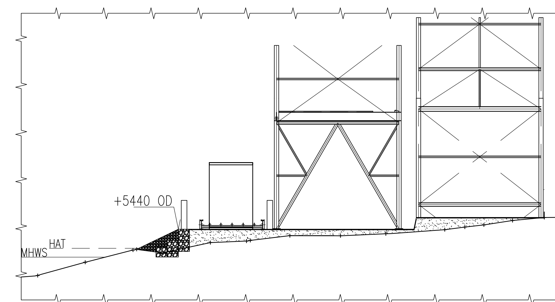
SECTION B-B FROM SKETCH 33605-S056
