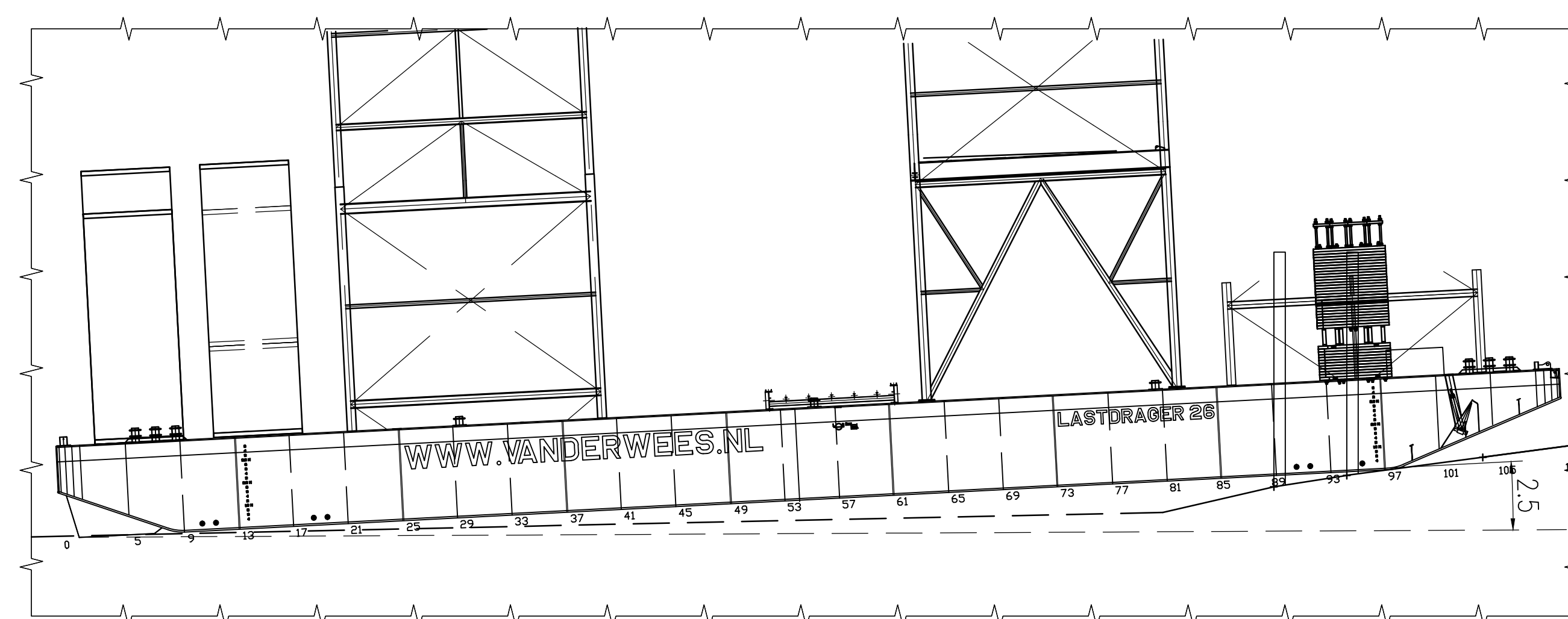
BARGE ANGLE WHEN LANDED AT <4,000 CD
