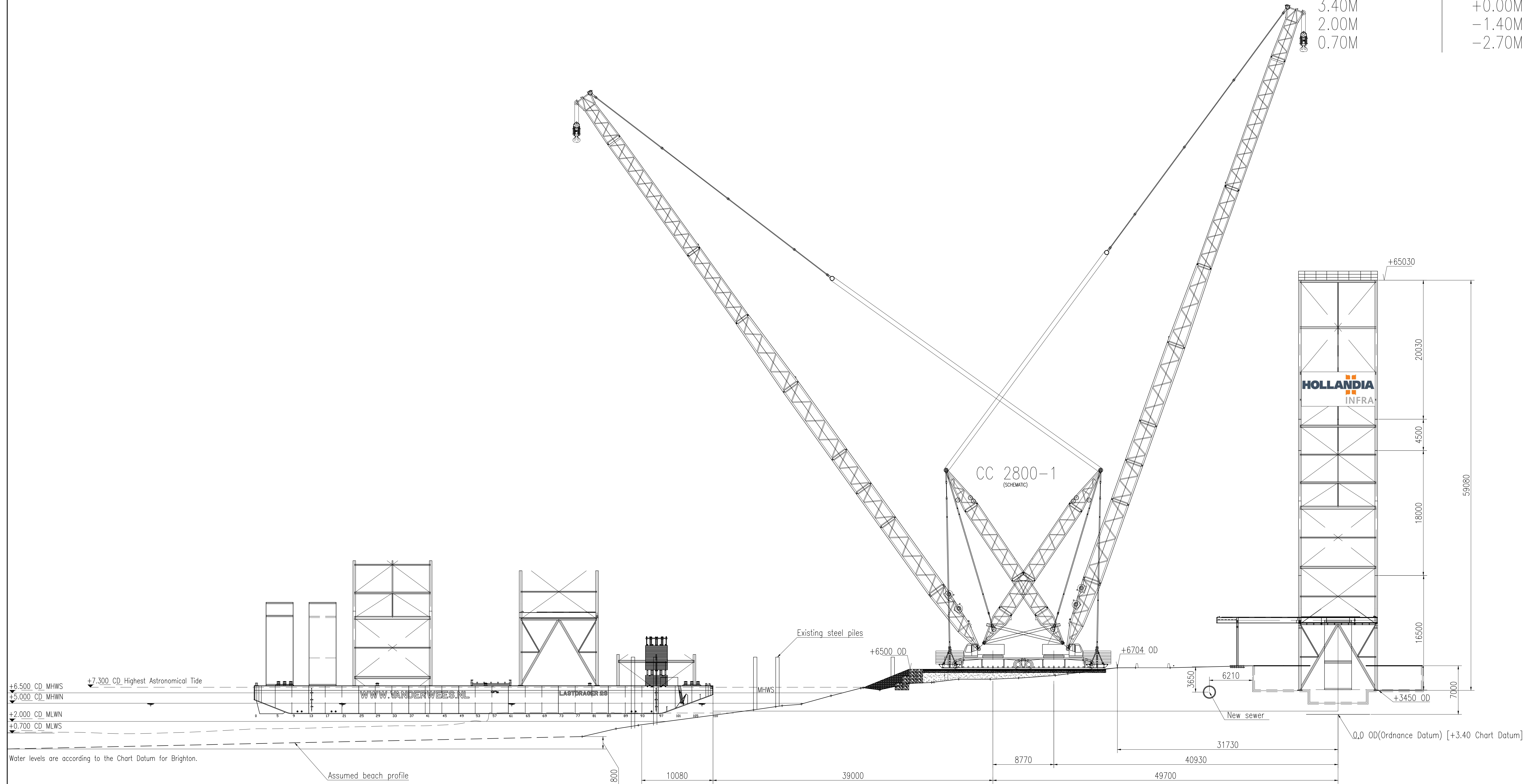
SECTION A-A FROM SKETCH 33605-S056
