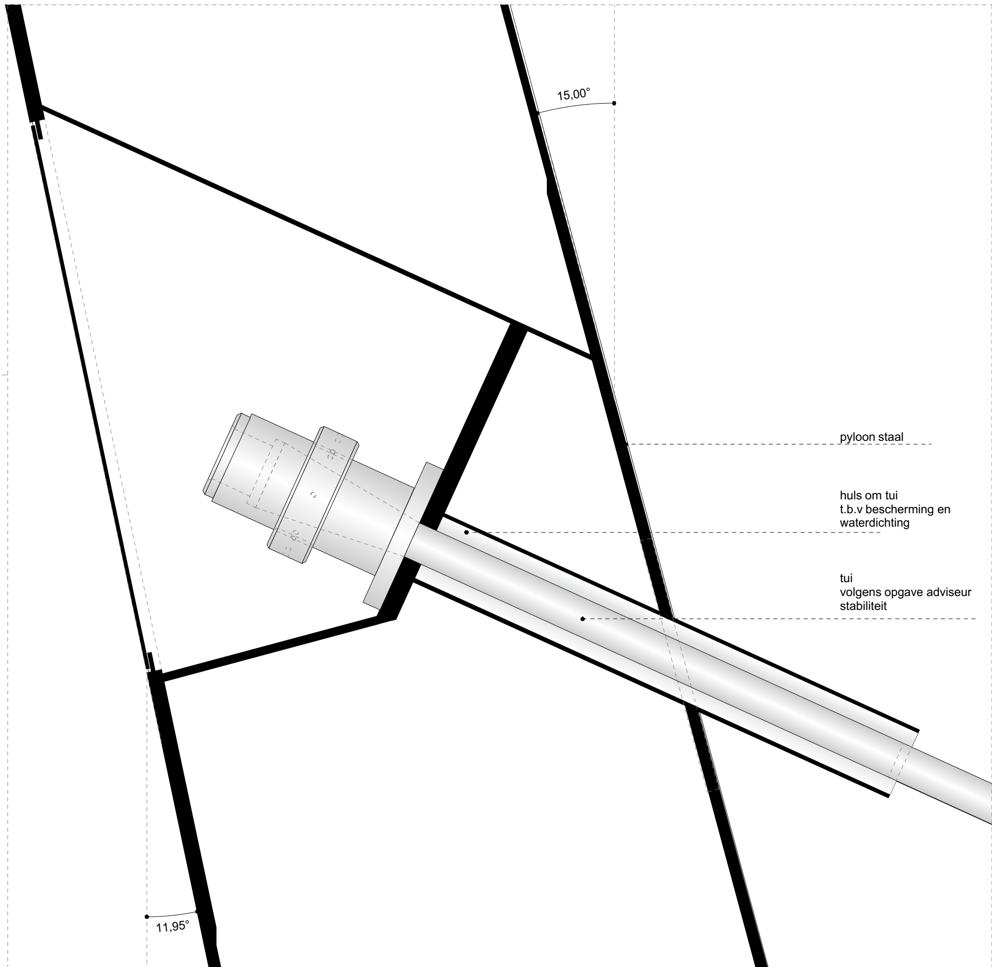
Detail C-C 1:75/10
