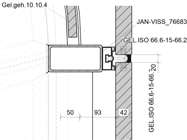
Detail H8 1:5
