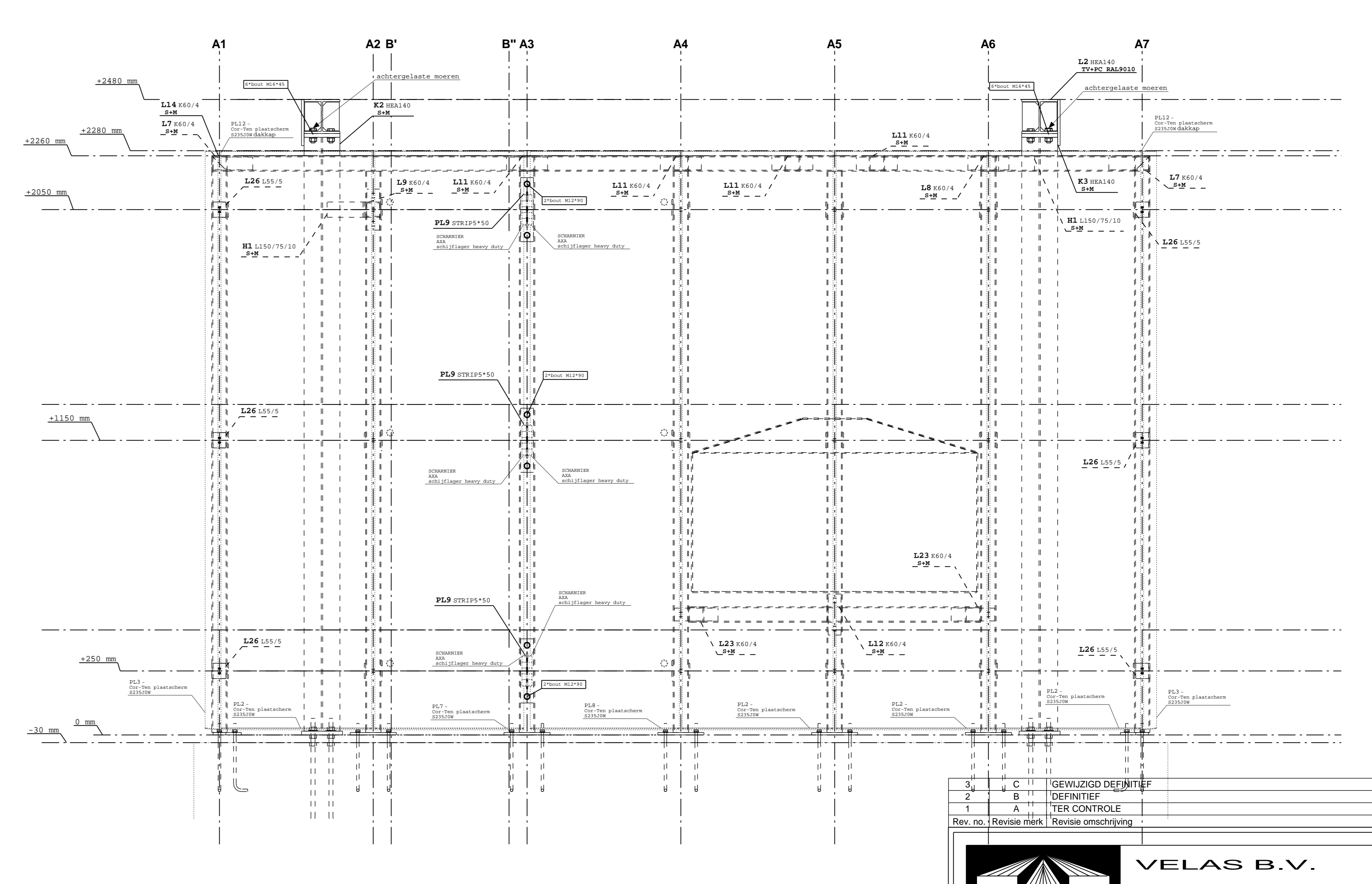
dsn K-K, 1:10
