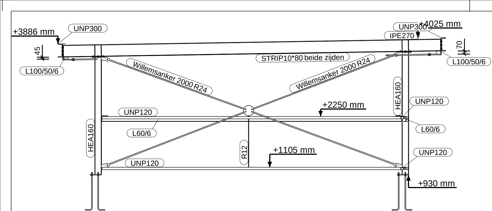
AANZICHT AS As 1:50
