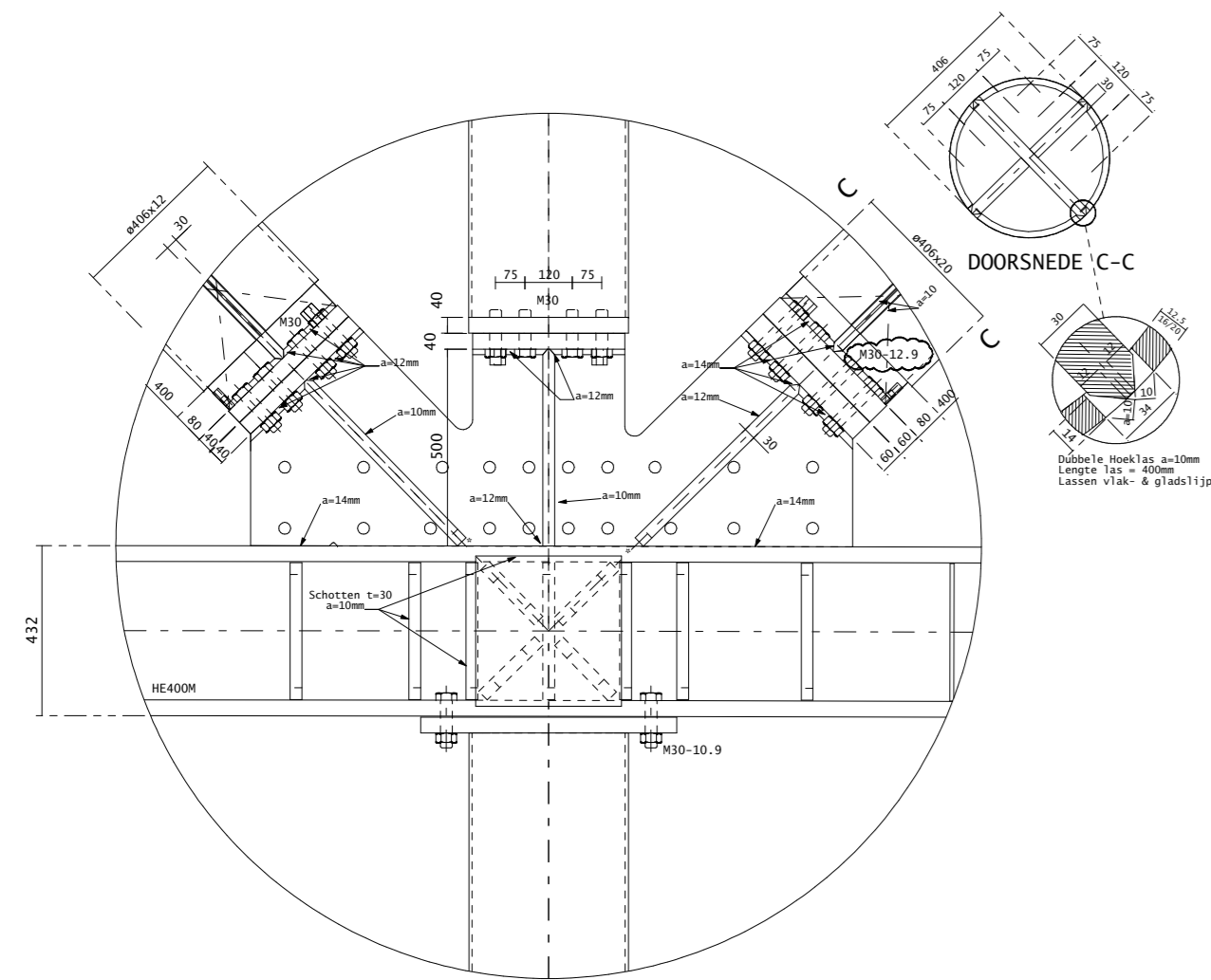
DETAIL VERBINDING
