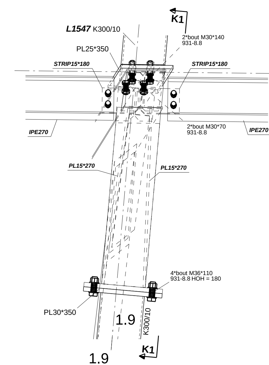
DETAIL K (1:15)
