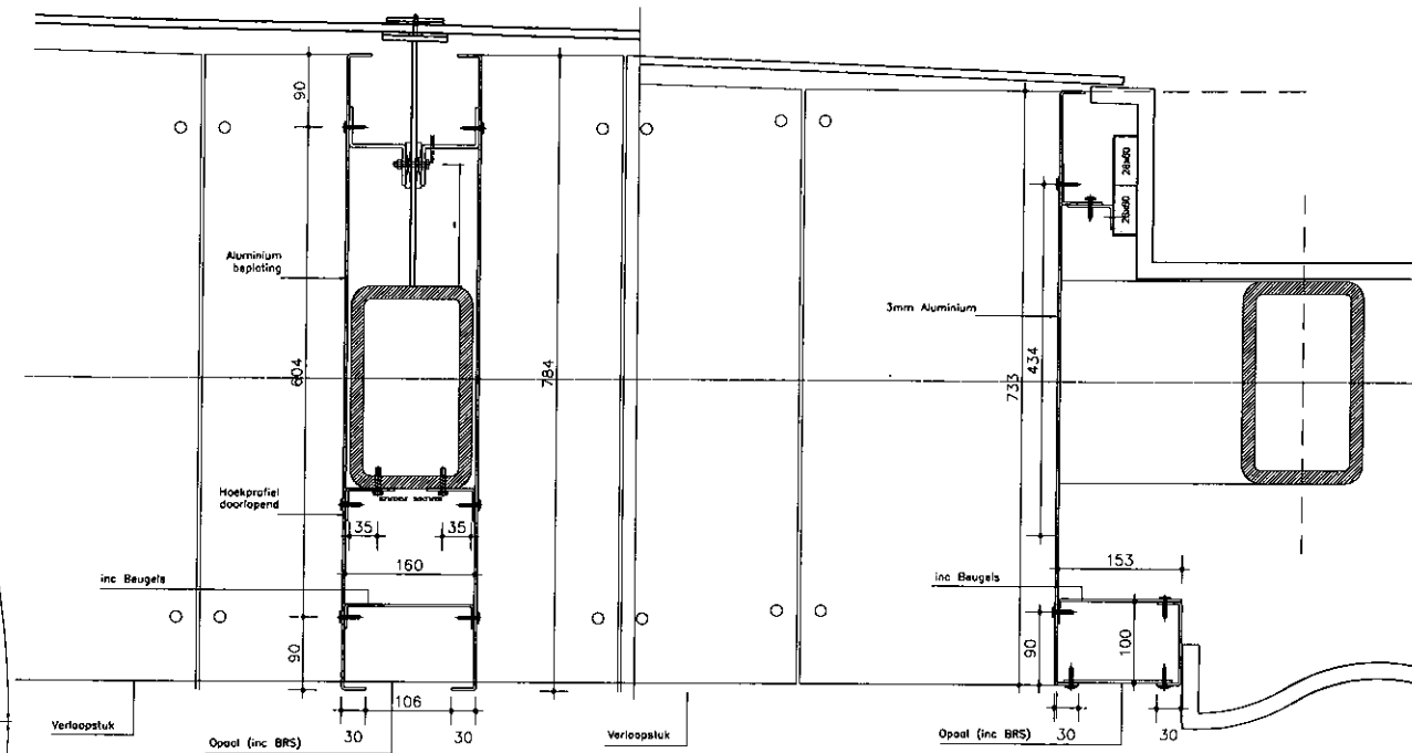
Detail 1 1:5
