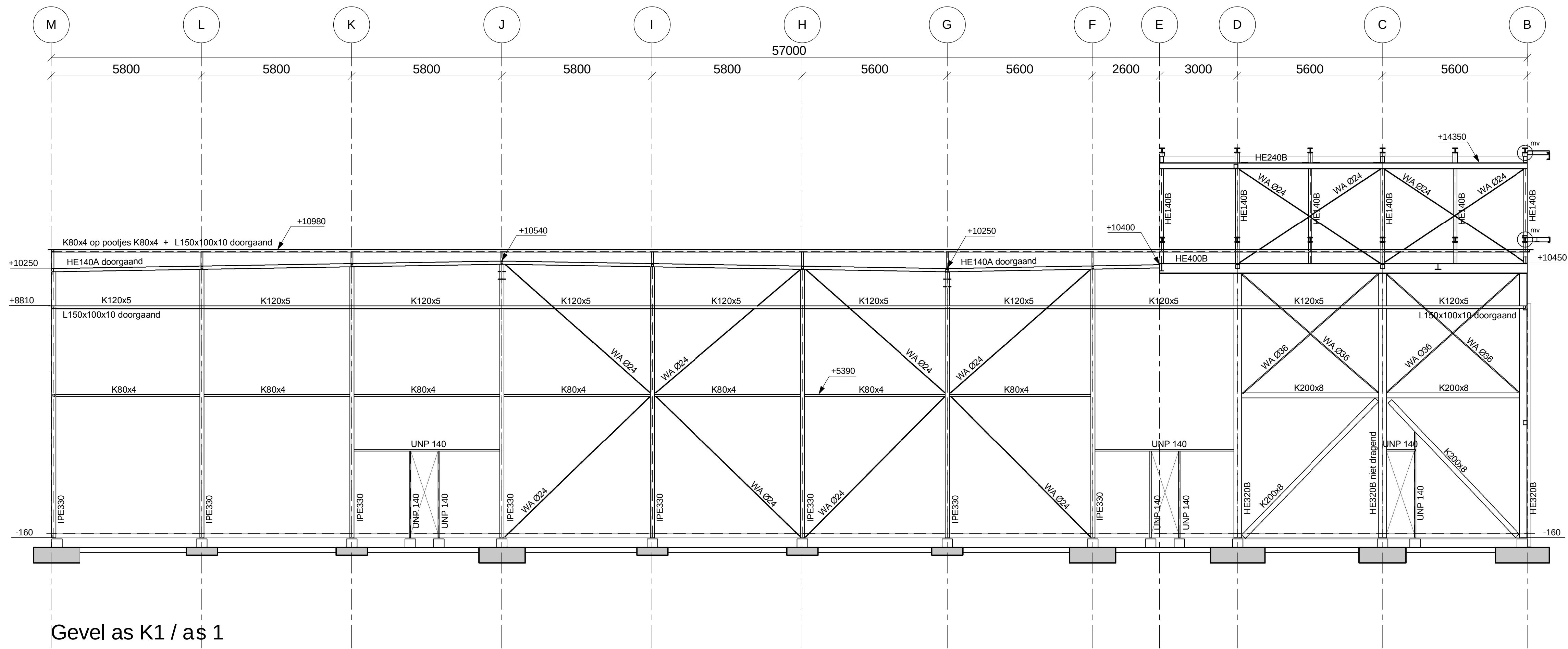
Gevel as K1 / as 1
