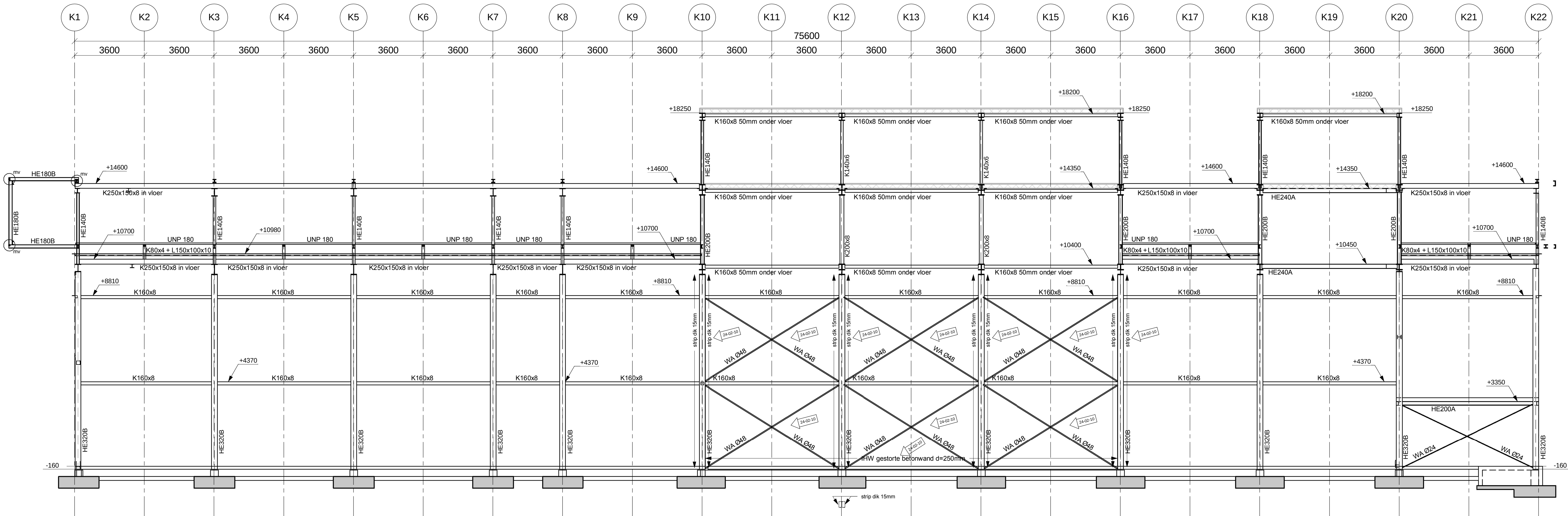
Gevel as B
