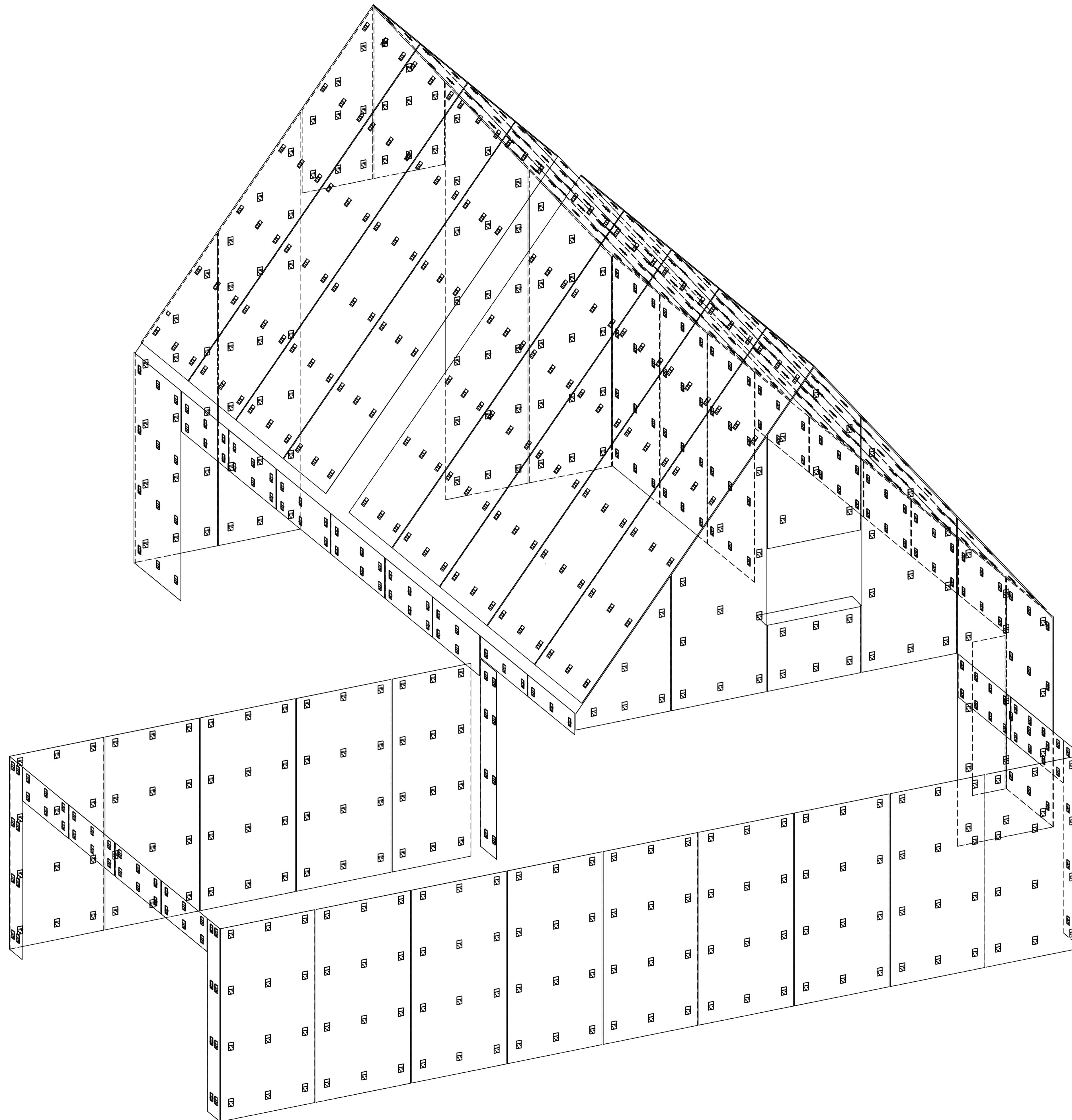
Model View Isometric view_4 (Sc1:30)
