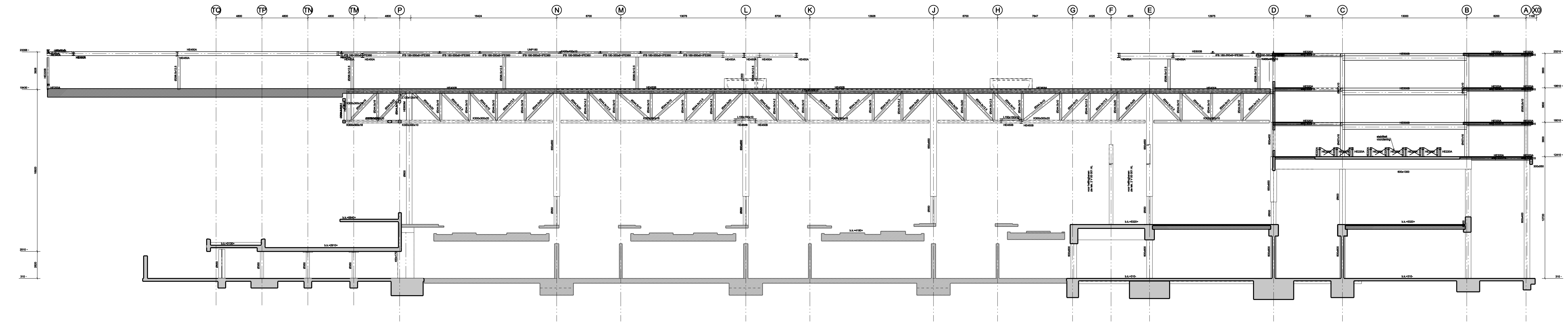
Doorsnede as 16
