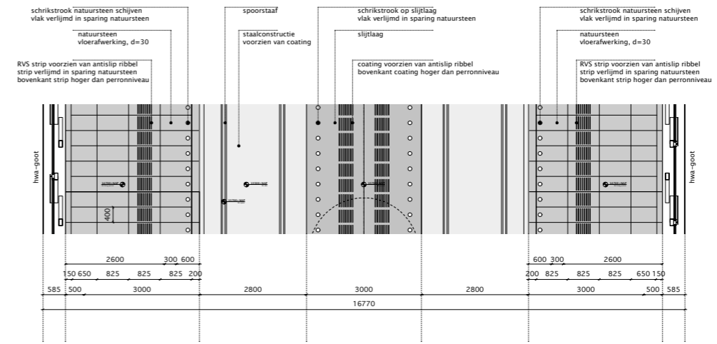
fragment A
