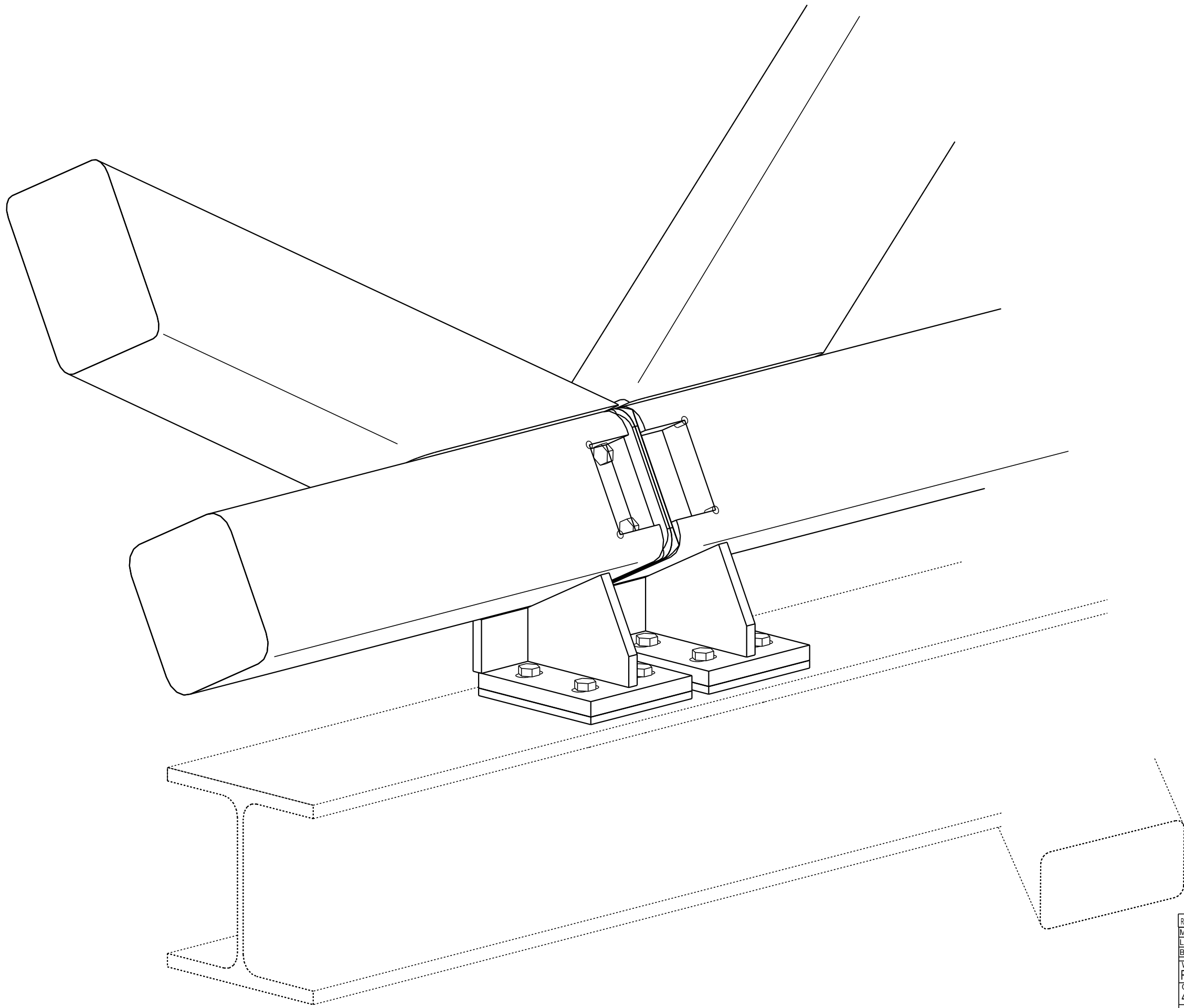
3D Detail 4 1:5
