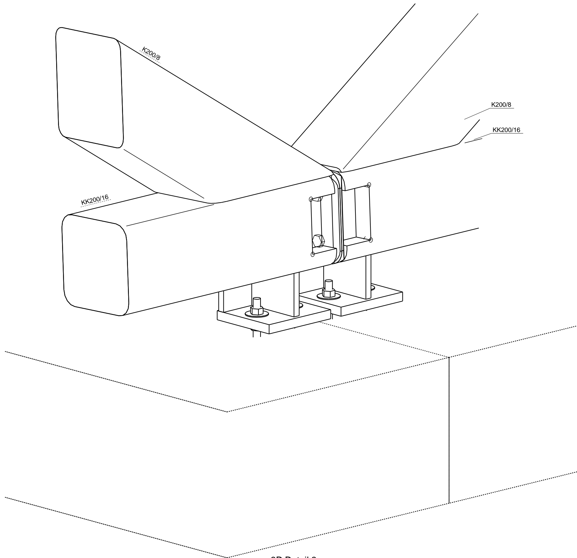
3D Detail 3 1:5
