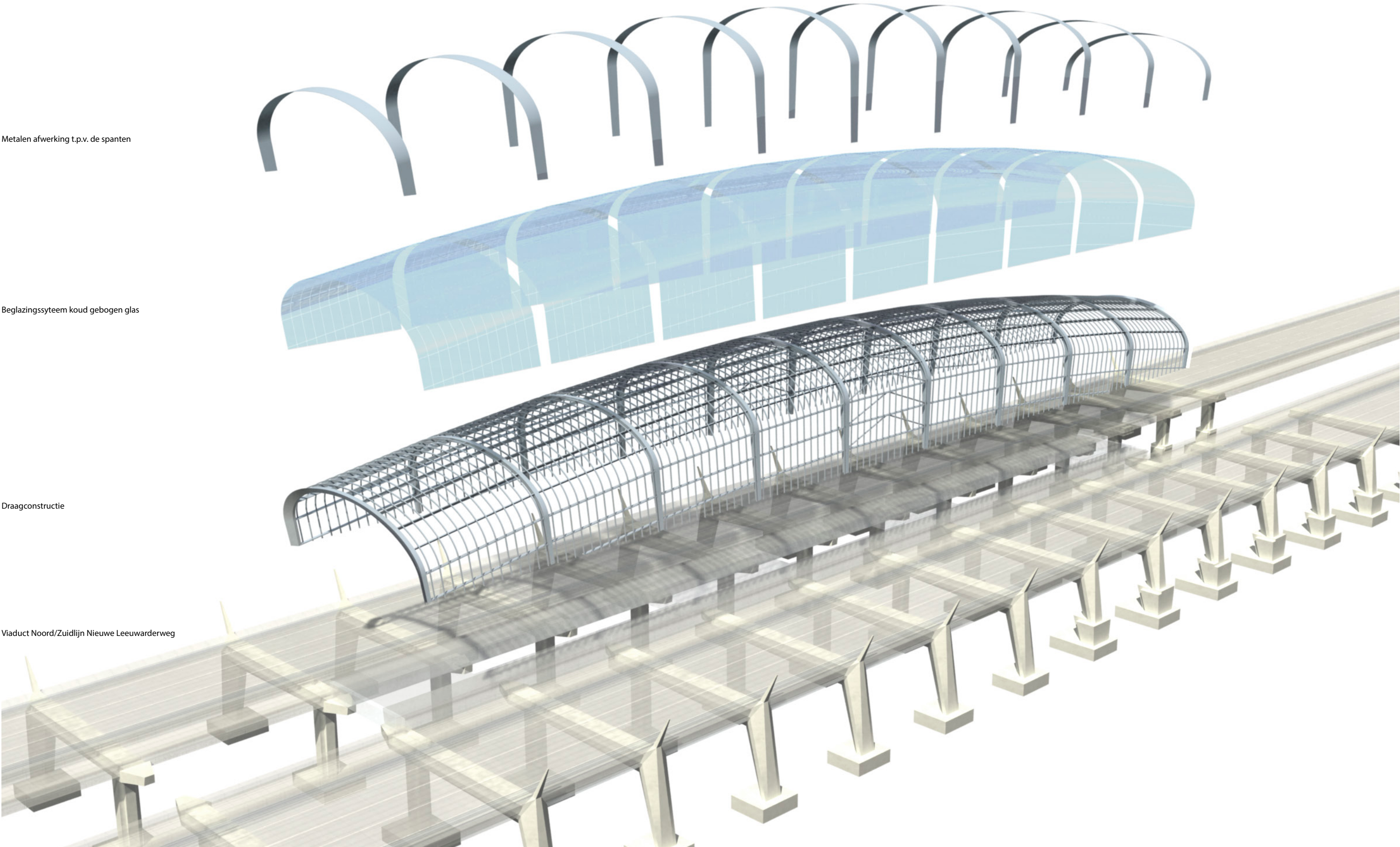
Exploded view
