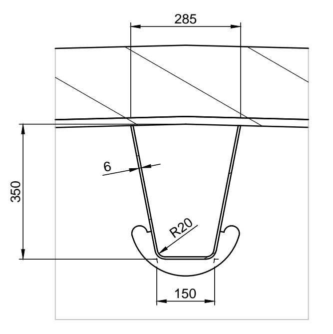
Detail 1 (1:10)
