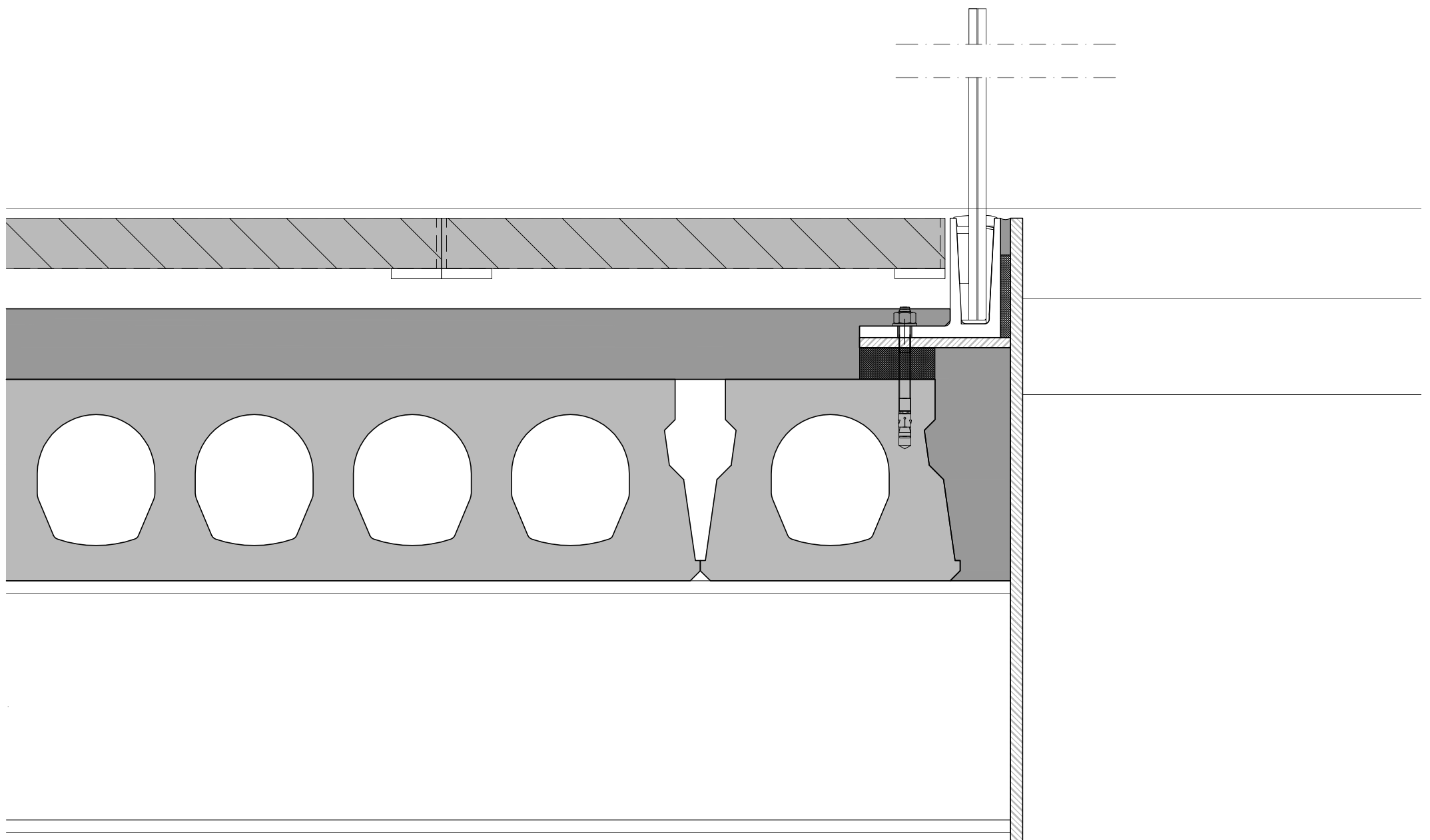
Detail luifel
