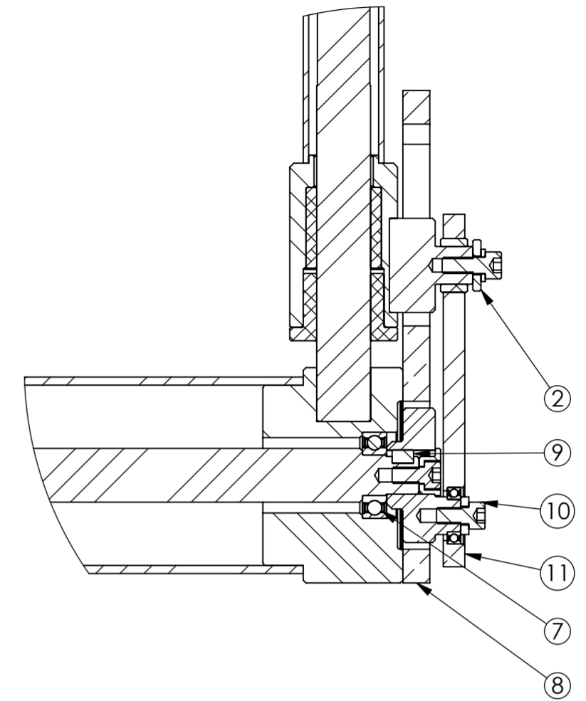
DETAIL B SCALE 1 : 2
