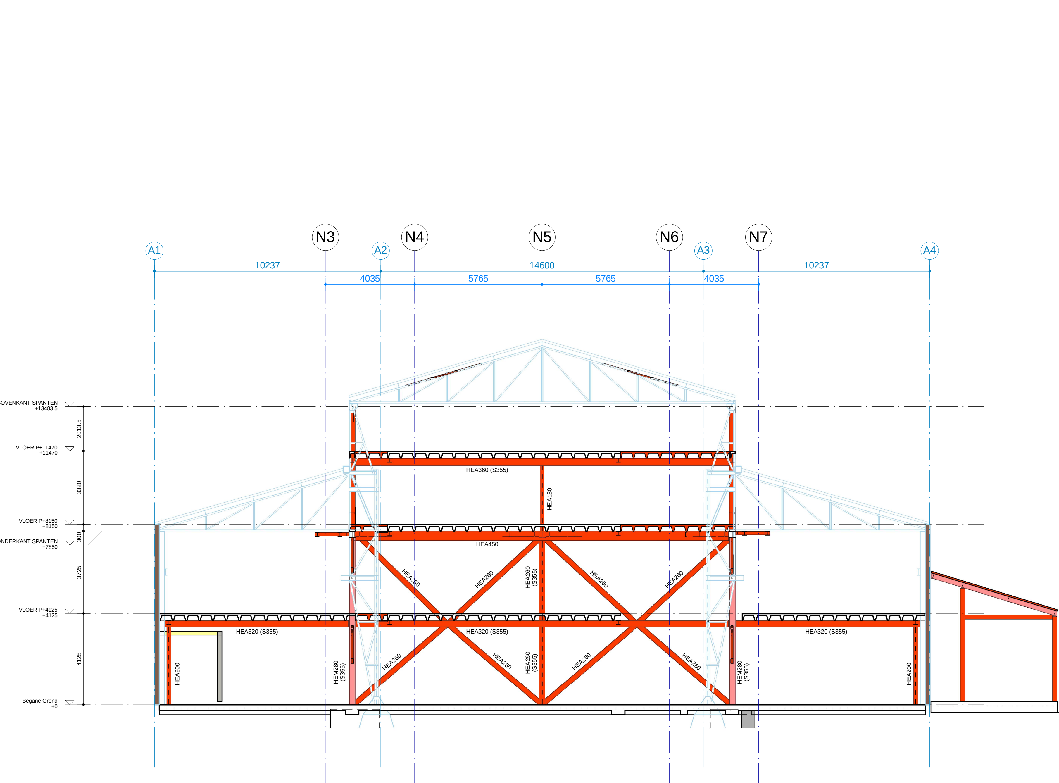
Doorsnede as AK Schaal: 1 : 100
