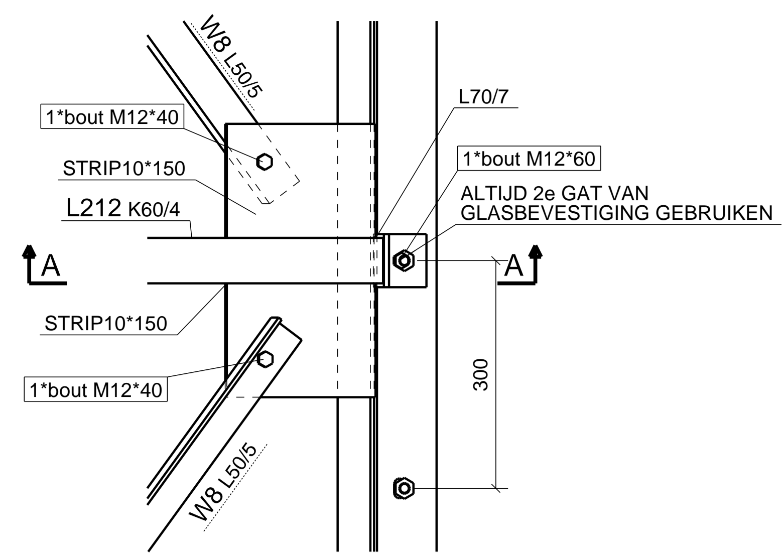
Detail 1, 1:10
