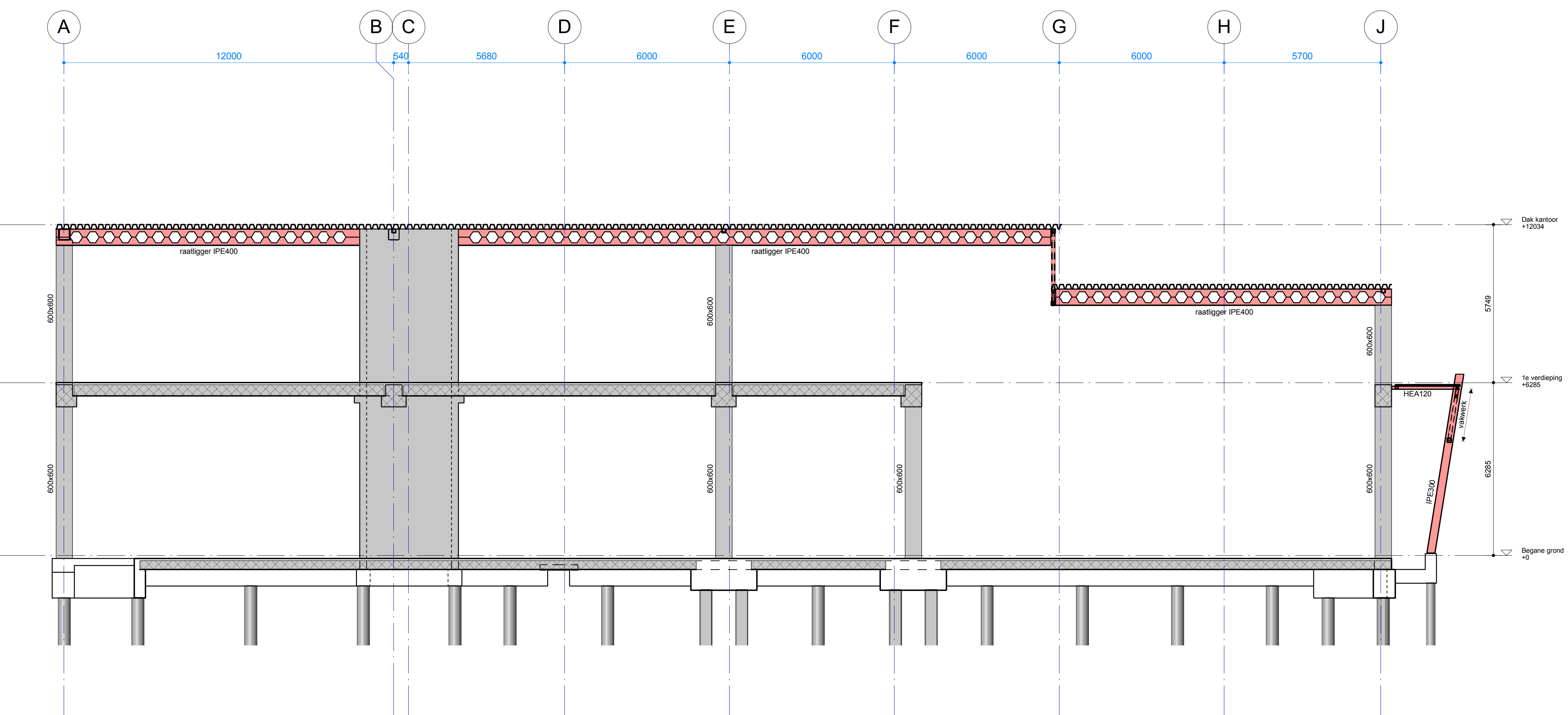
Doorsnede as 08
