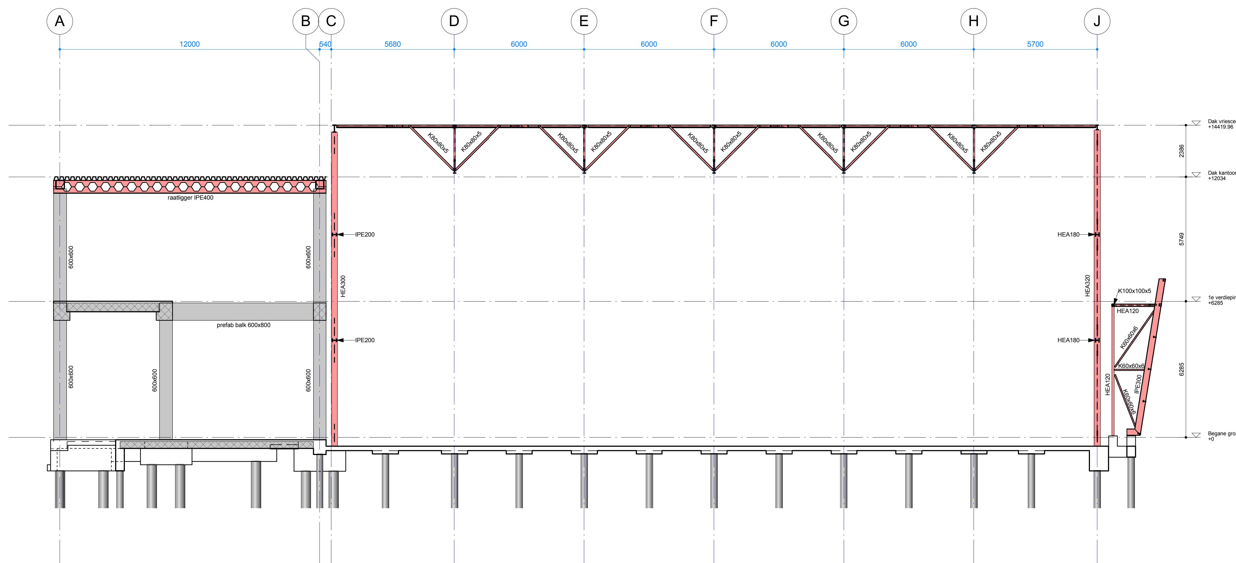
Doorsnede as 03
