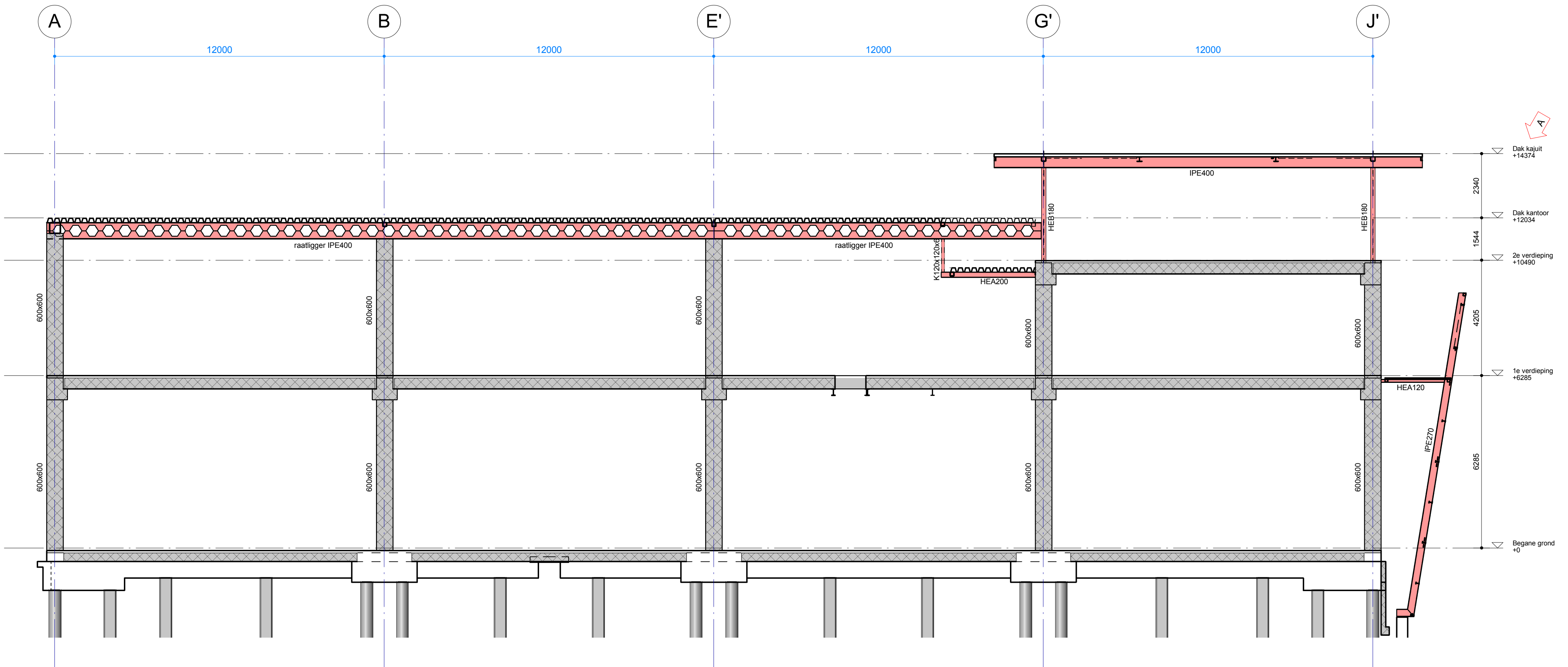
Doorsnede as 13
