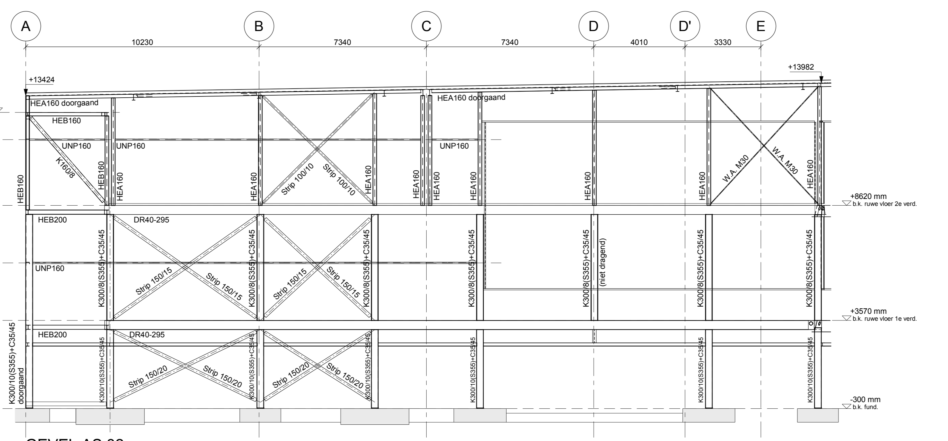
GEVEL AS 32
