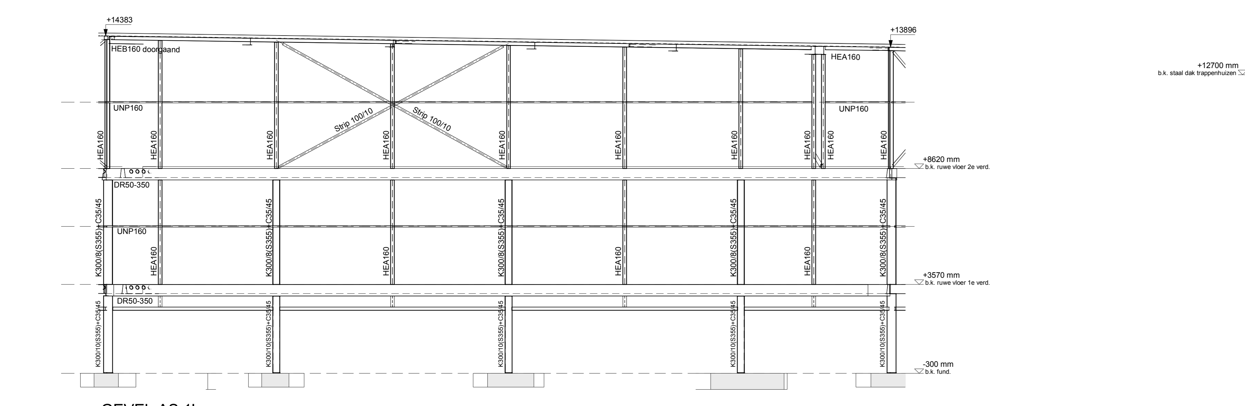
GEVEL AS 1'
