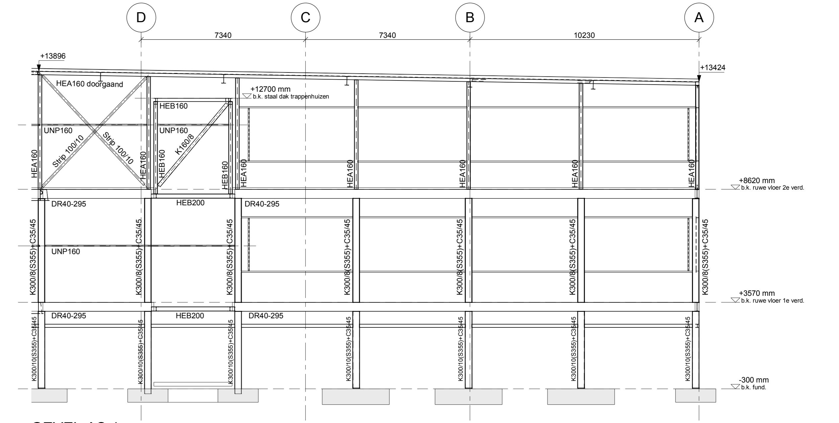
GEVEL AS 1
