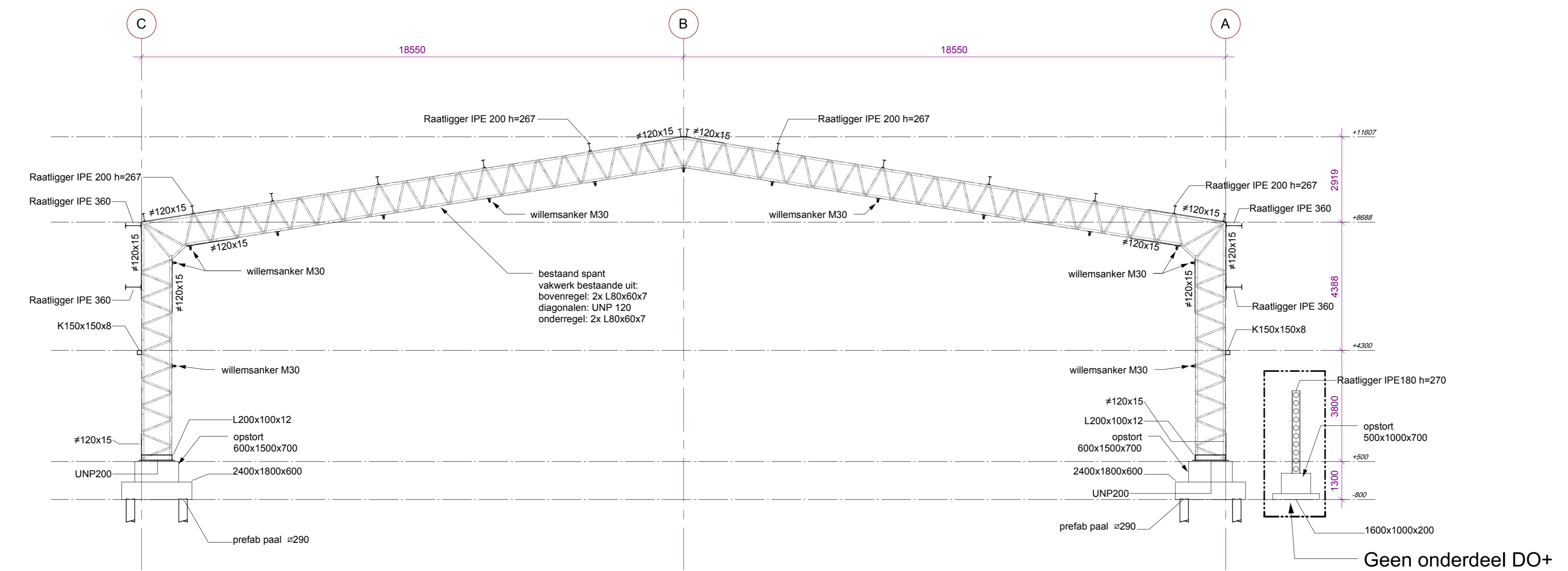
doorsnede as 6 1 : 100
