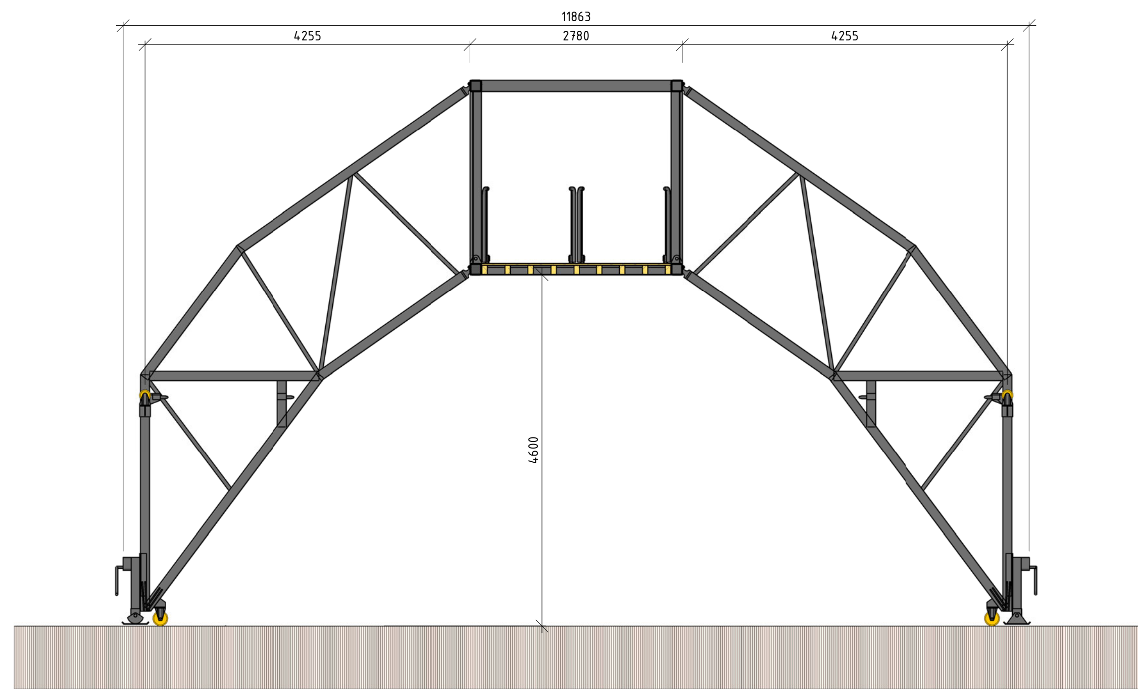
3 Cross-section of two EventBridges mounted in one line with stairways parallel to the body scale
