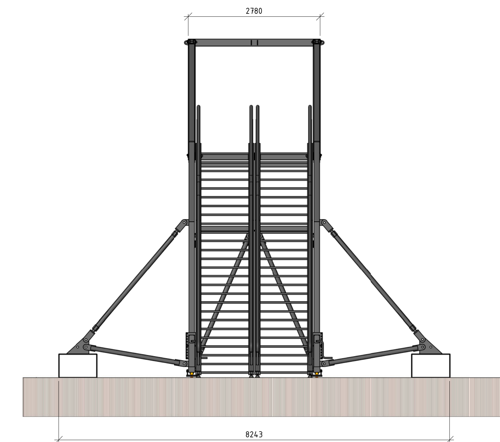
4 Front view of two EventBridges mounted in one line with stairways parallel to the body scale
