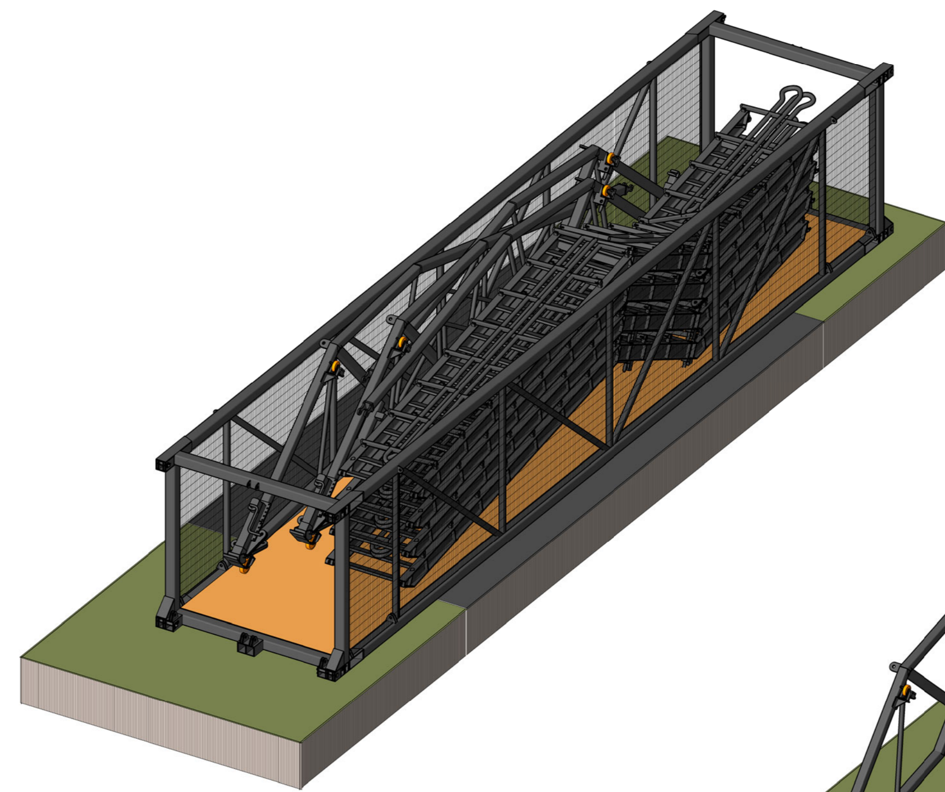
2 Unloading of EventBridge scale
