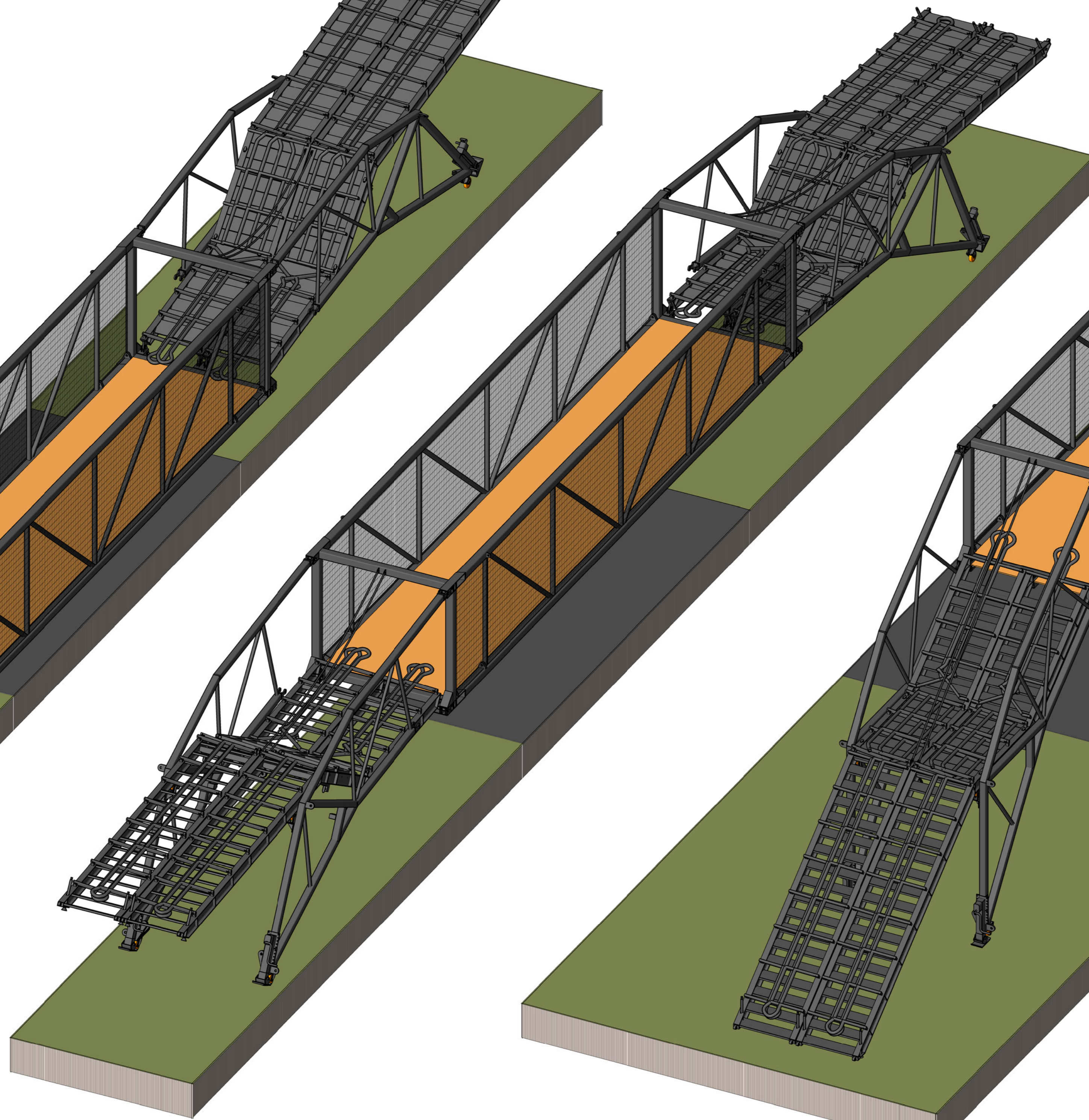
5 Lifting the entire structure scale
