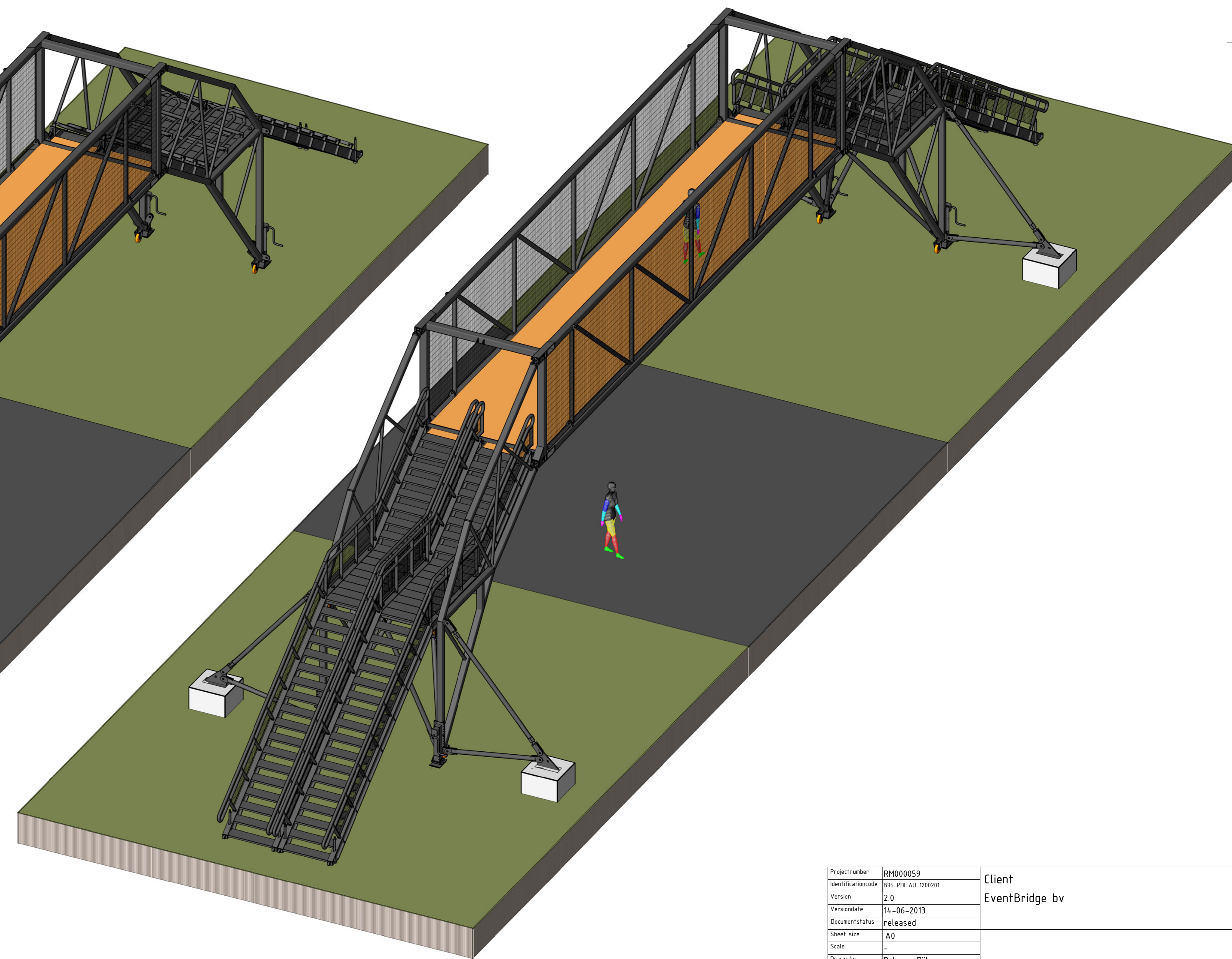
7 Erected EventBridge with stairways parallel to the body scale
