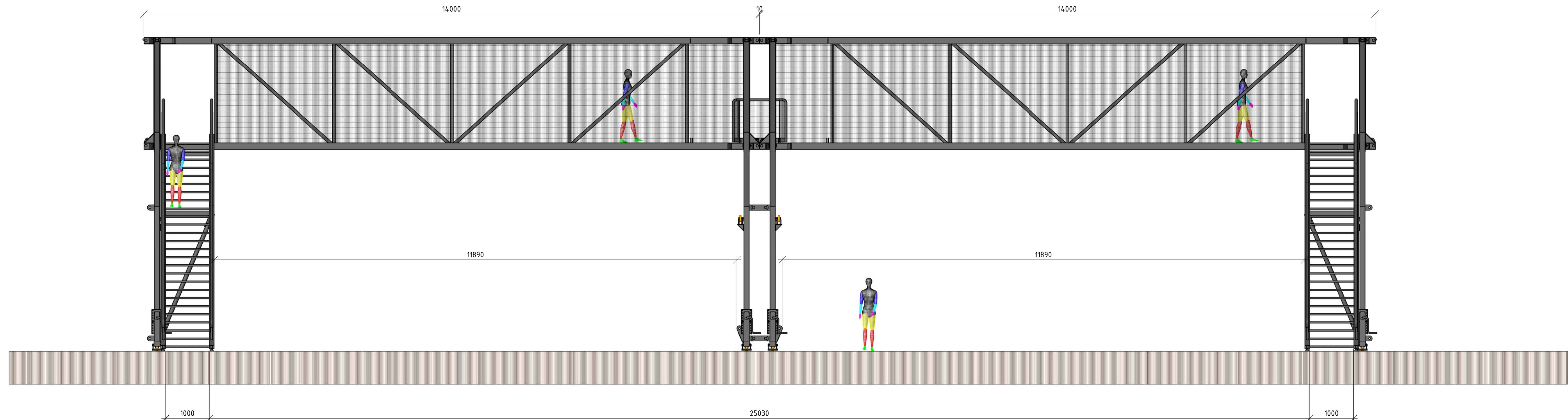
5 Side view of two EventBridges mounted in one line scale
