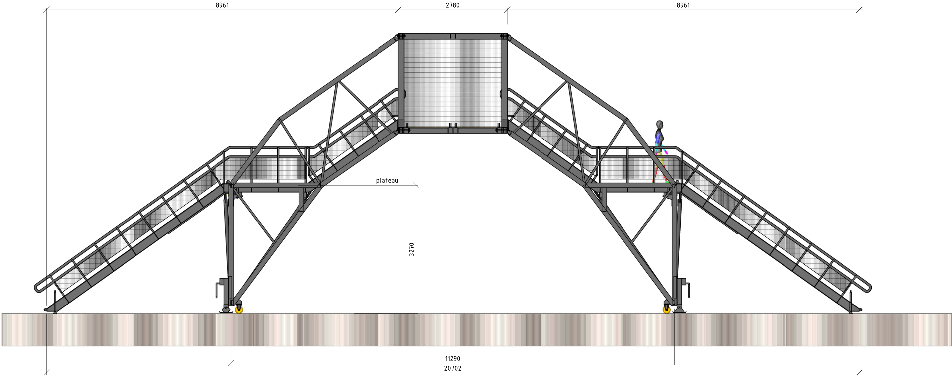
3 Front view of two EventBridges mounted in one line scale
