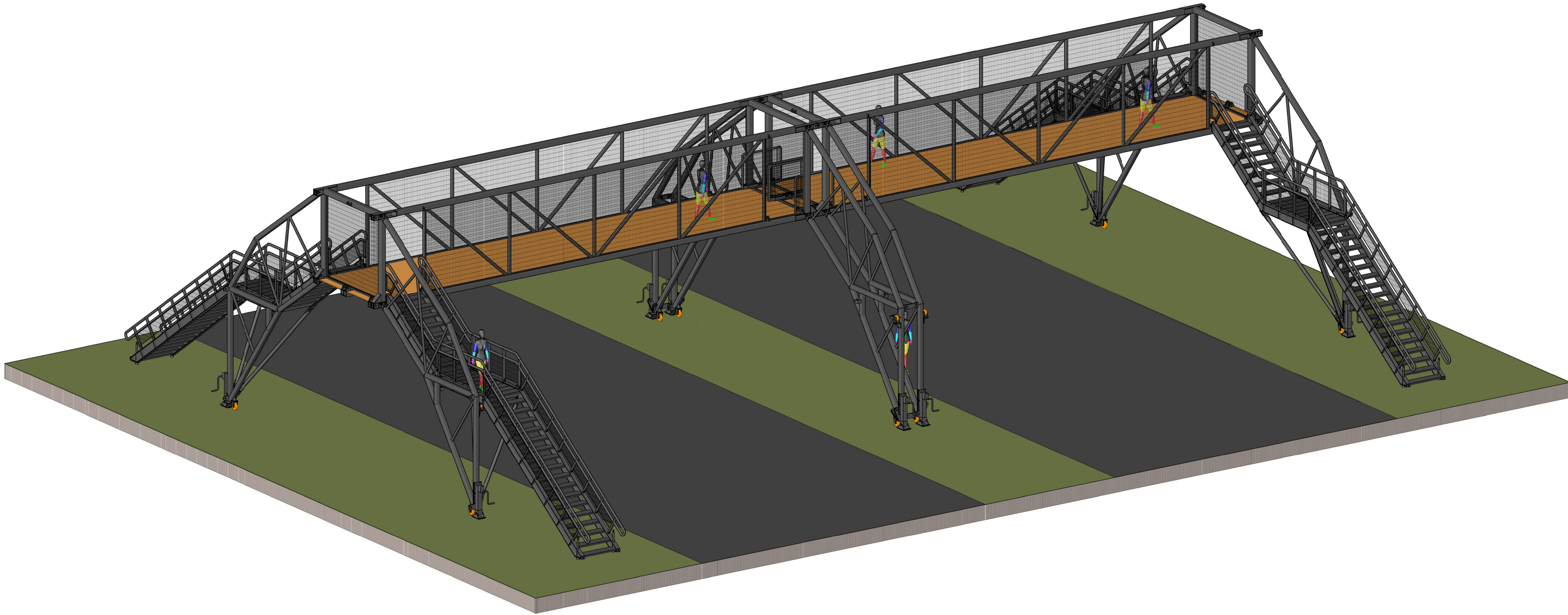
1 Isometric view of two EventBridges mounted in one line scale
