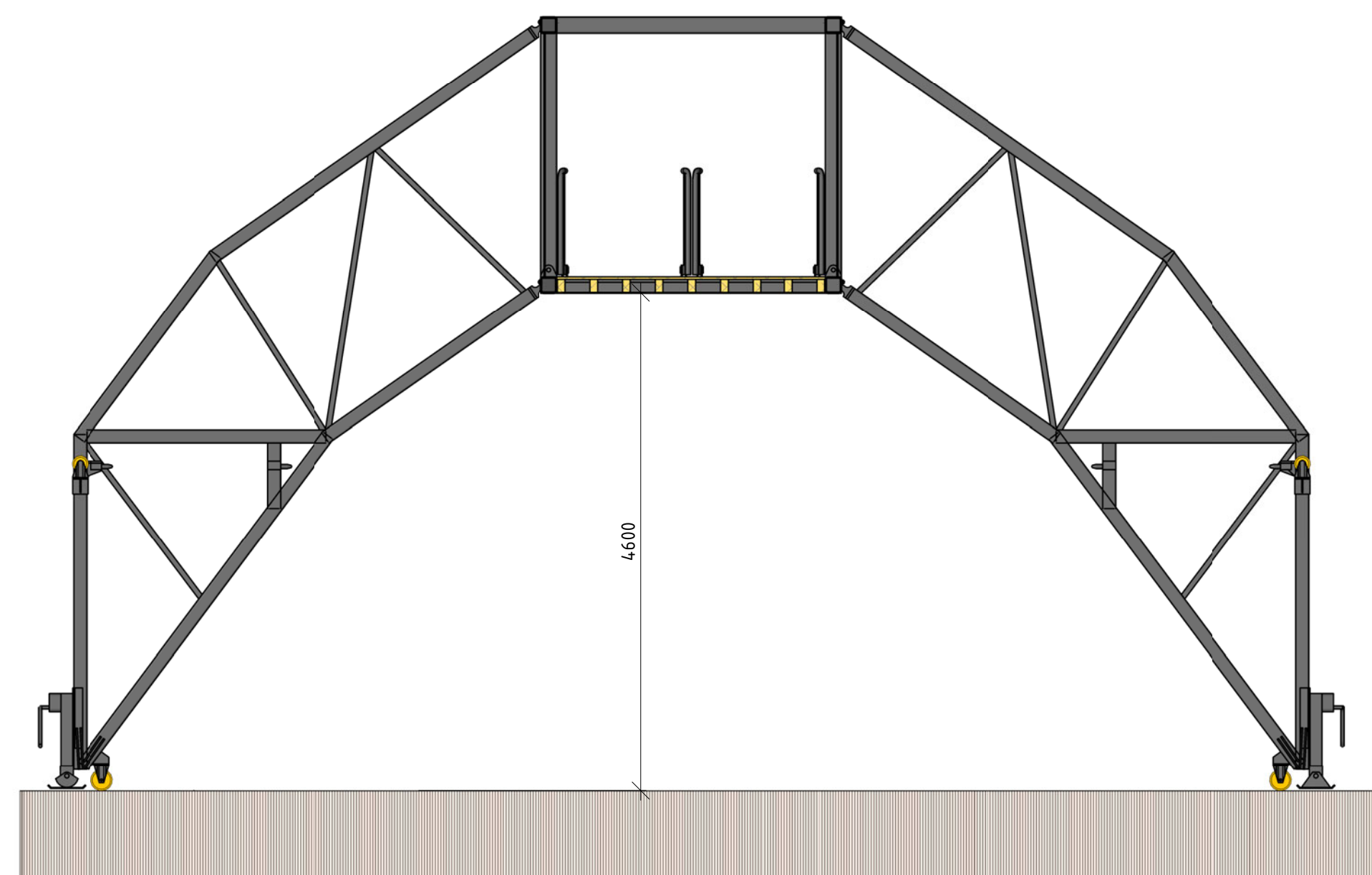
4 Cross-section of two EventBridges mounted in one line scale
