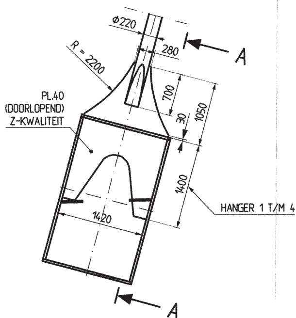
PRINCIPE DETAIL HANGER 1 T/M 4
