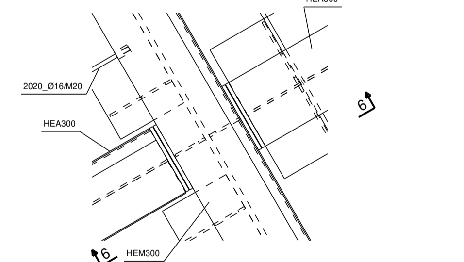
detail 6, 1:15
