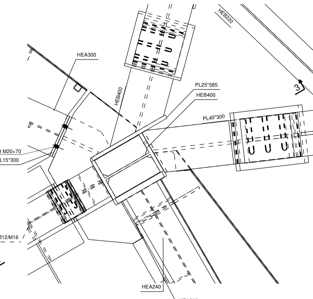
detail 3, 1:15
