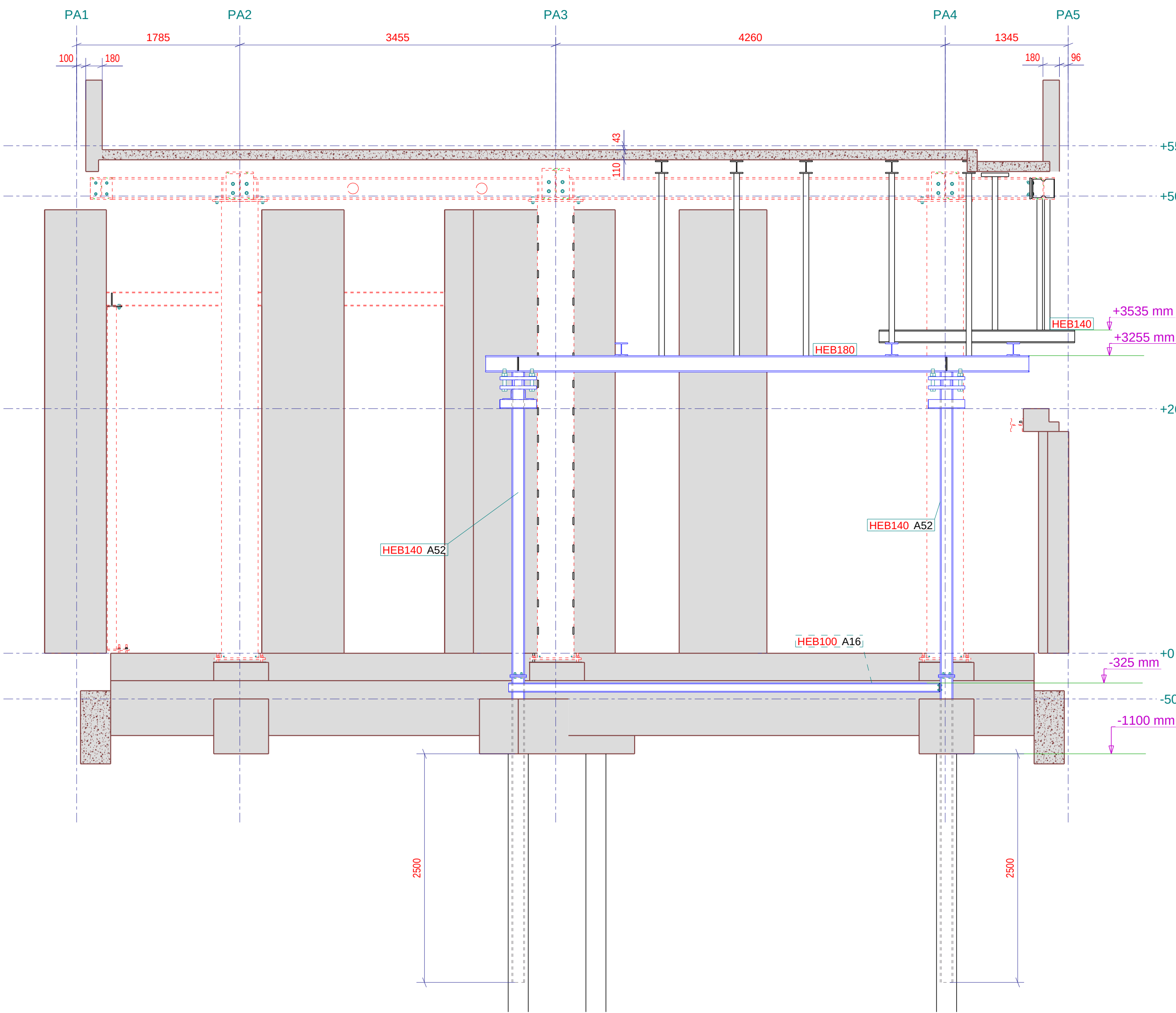
Aanzicht as P05 1:35
