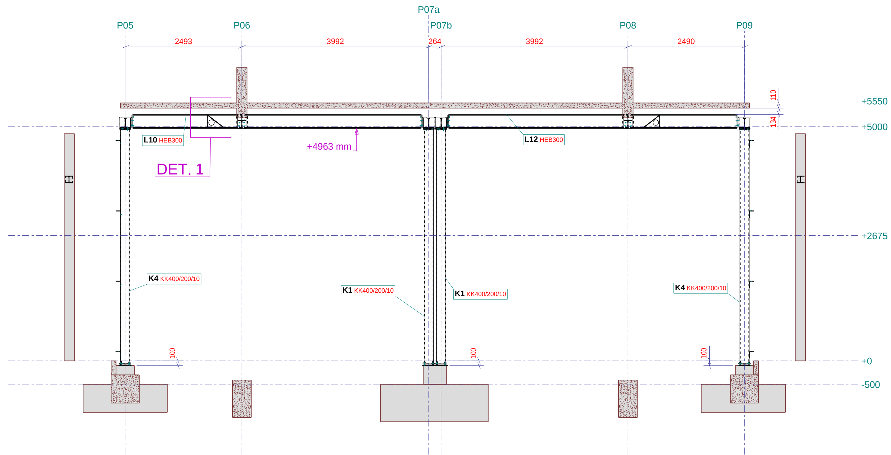
Aanzicht as PA2 1:50
