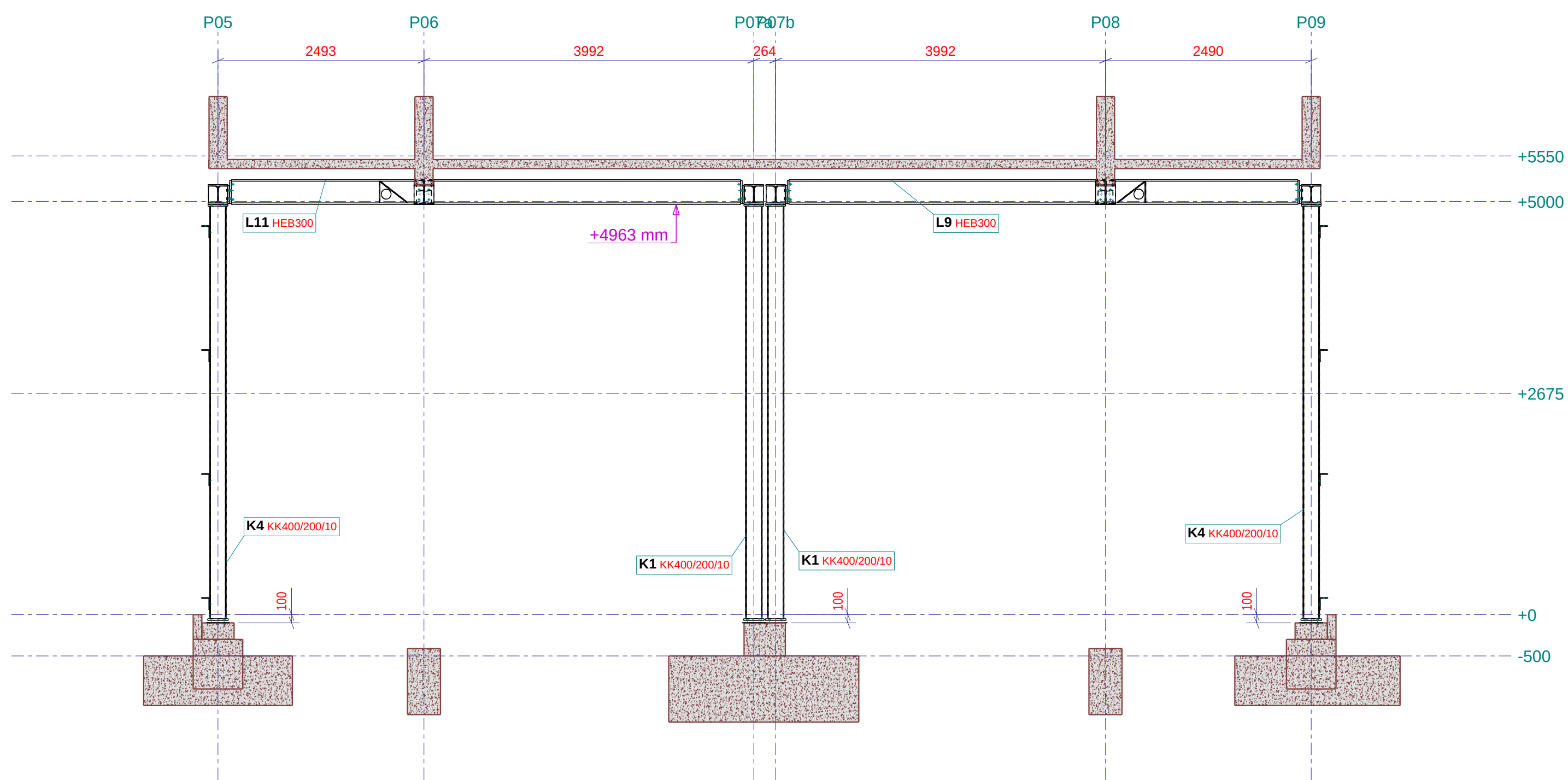
Aanzicht as PA4 1:50
