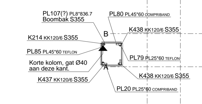
detail 3, 1:50
