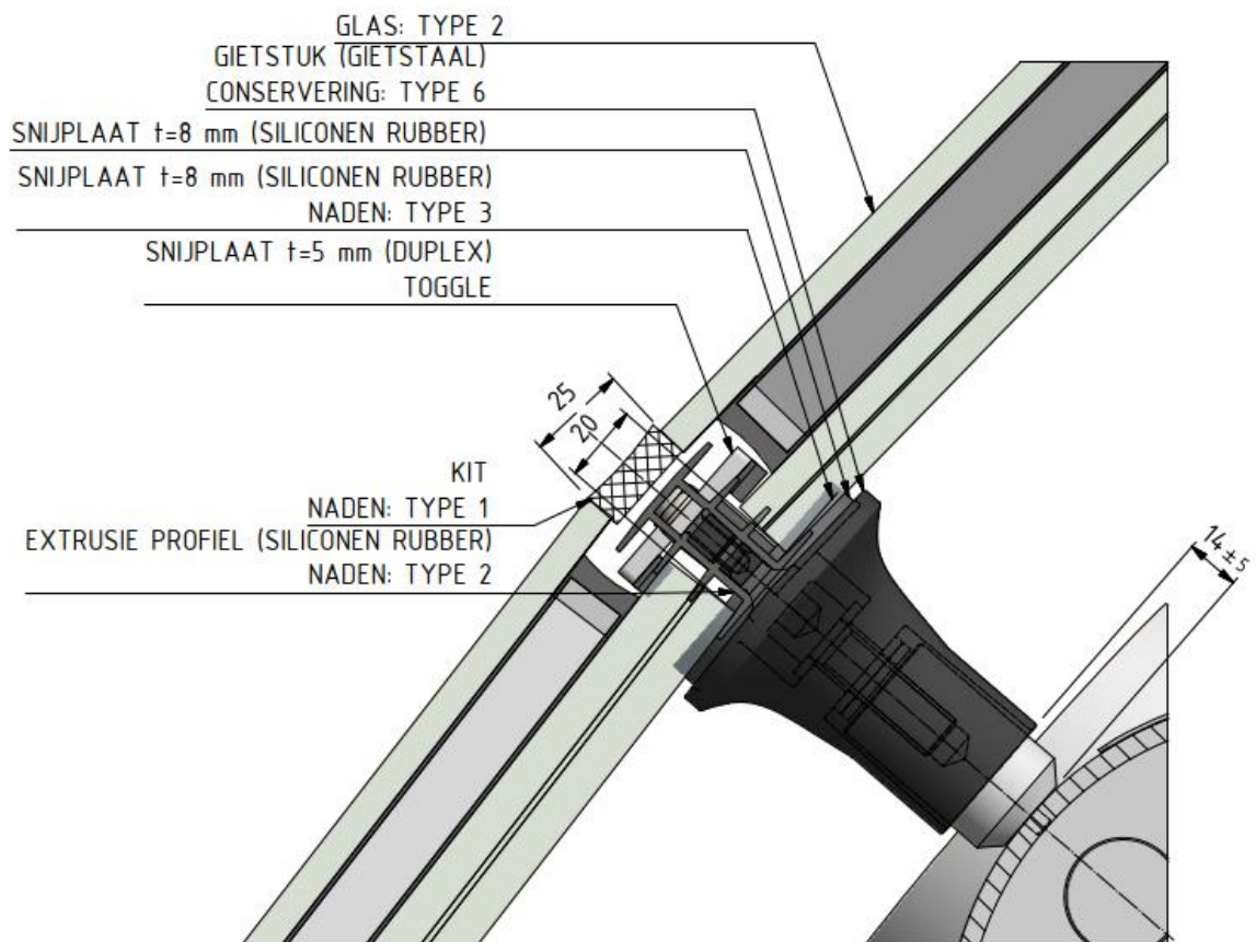
DETAIL X (1 : 2)
