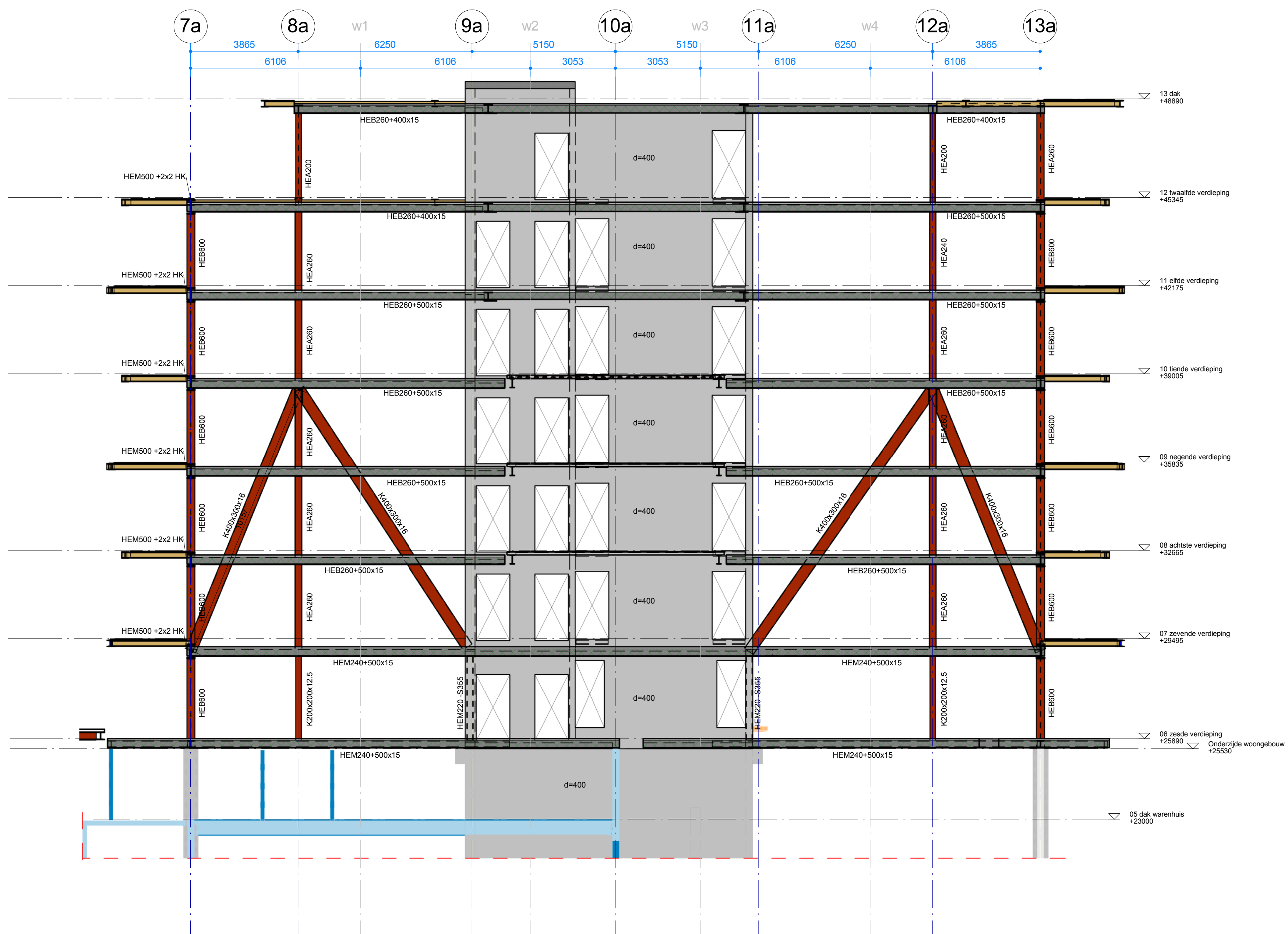
Doorsnede as N
