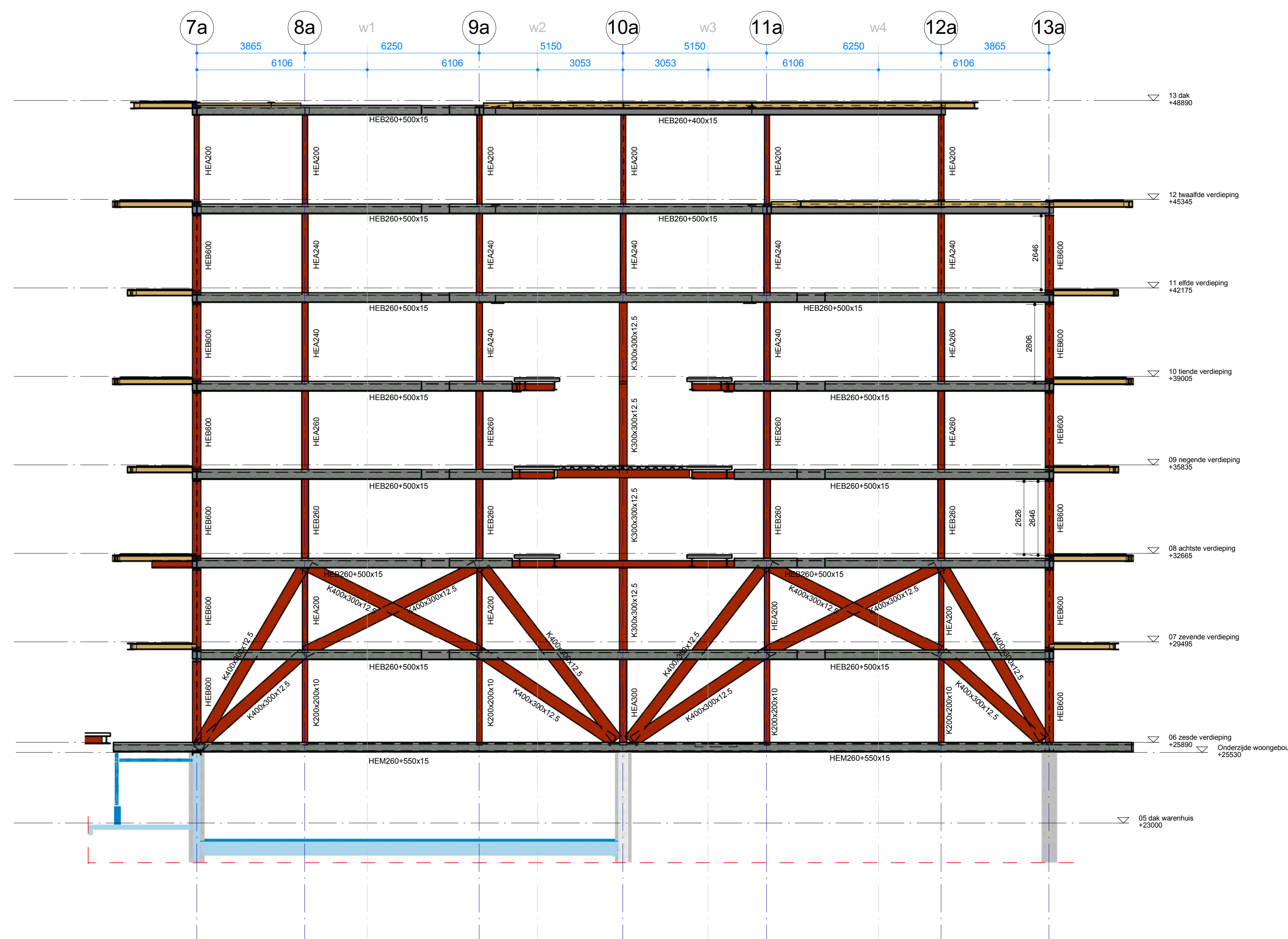
Doorsnede as L
