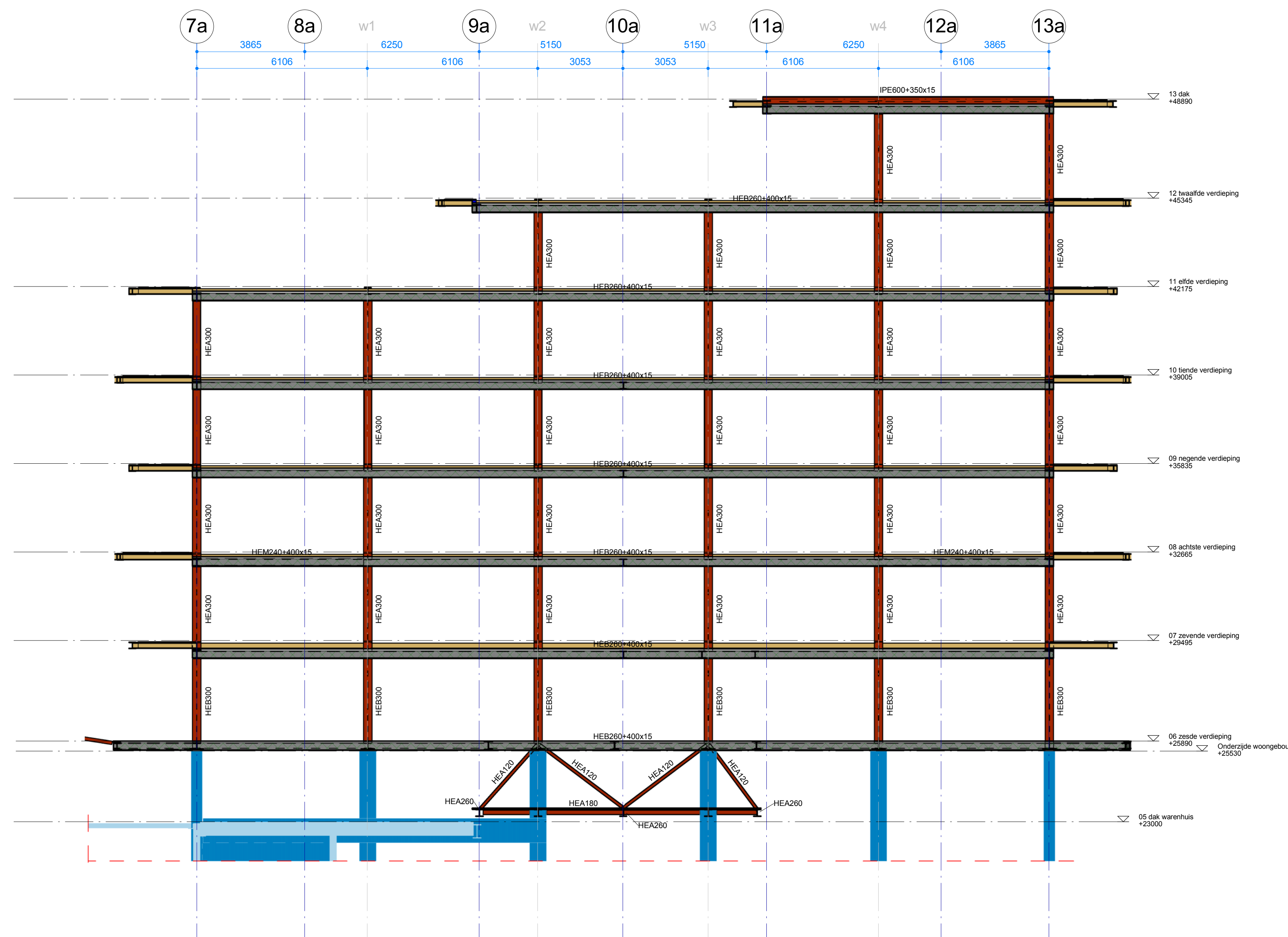
Doorsnede as Q (w6)
