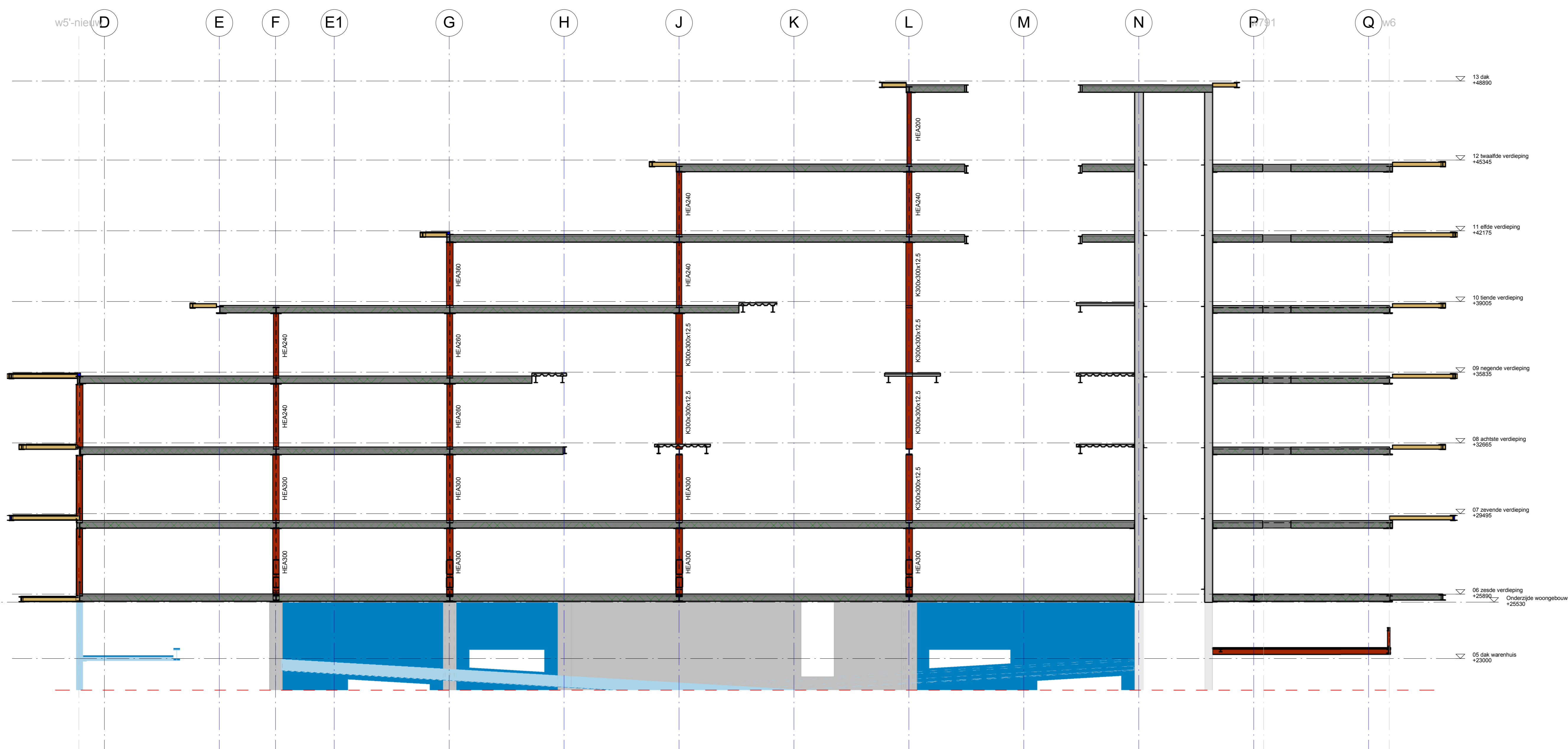
Doorsnede as 10A
