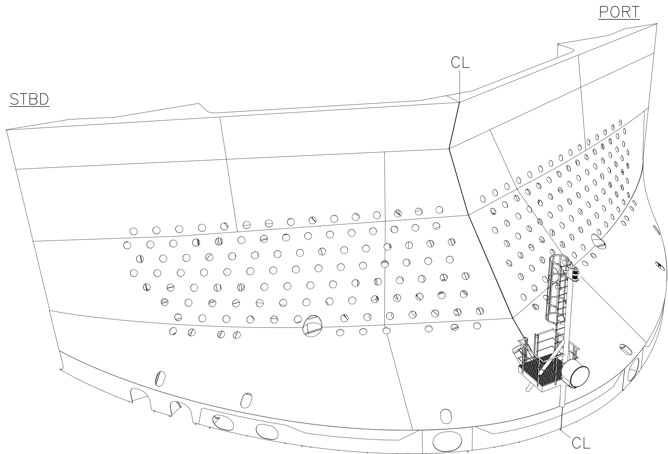
- BOW COVER ISO VIEW - LOOKING AFT / PORT
