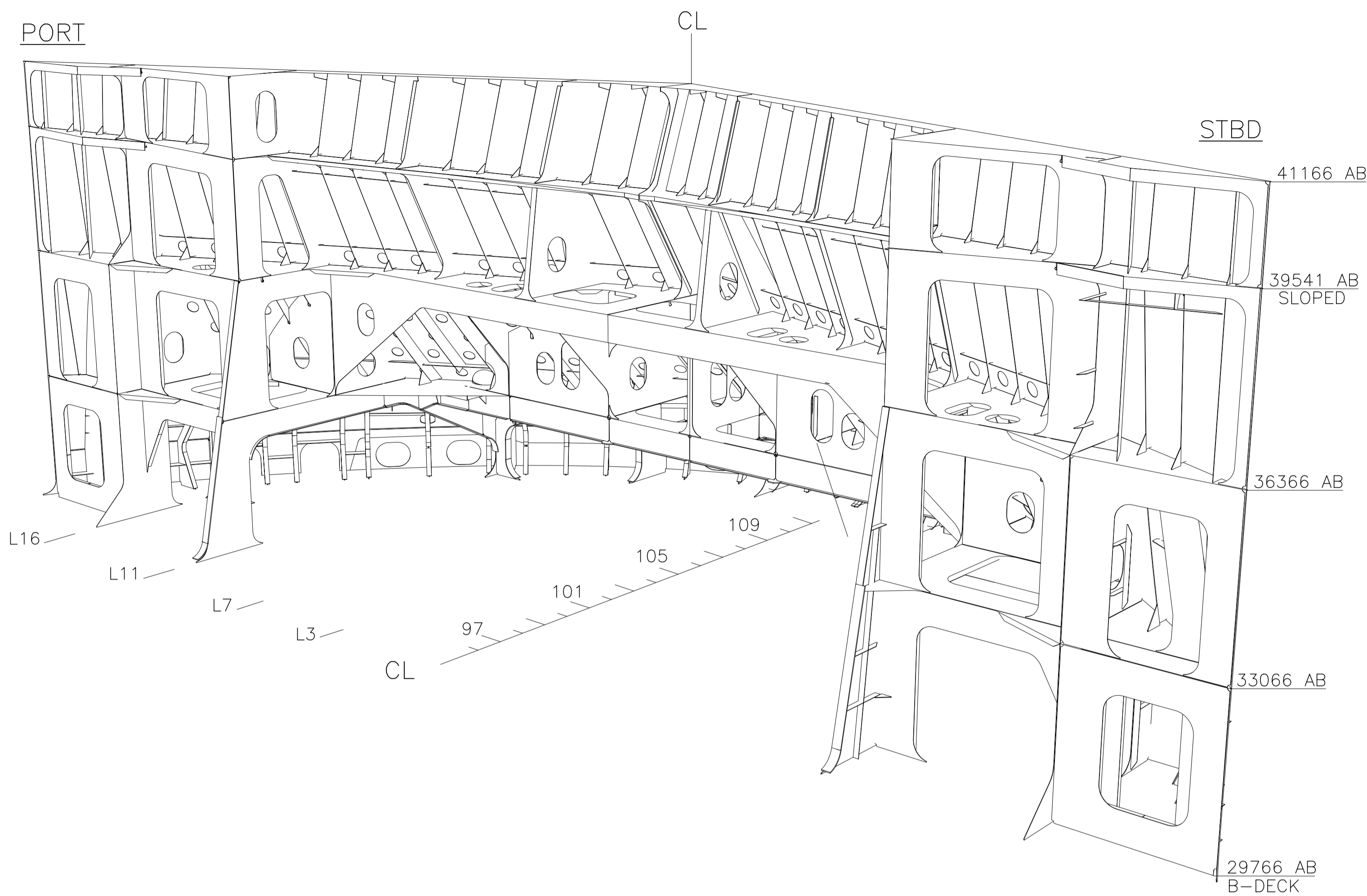
- BOW COVER ISO VIEW - LOOKING FWD / STBD
