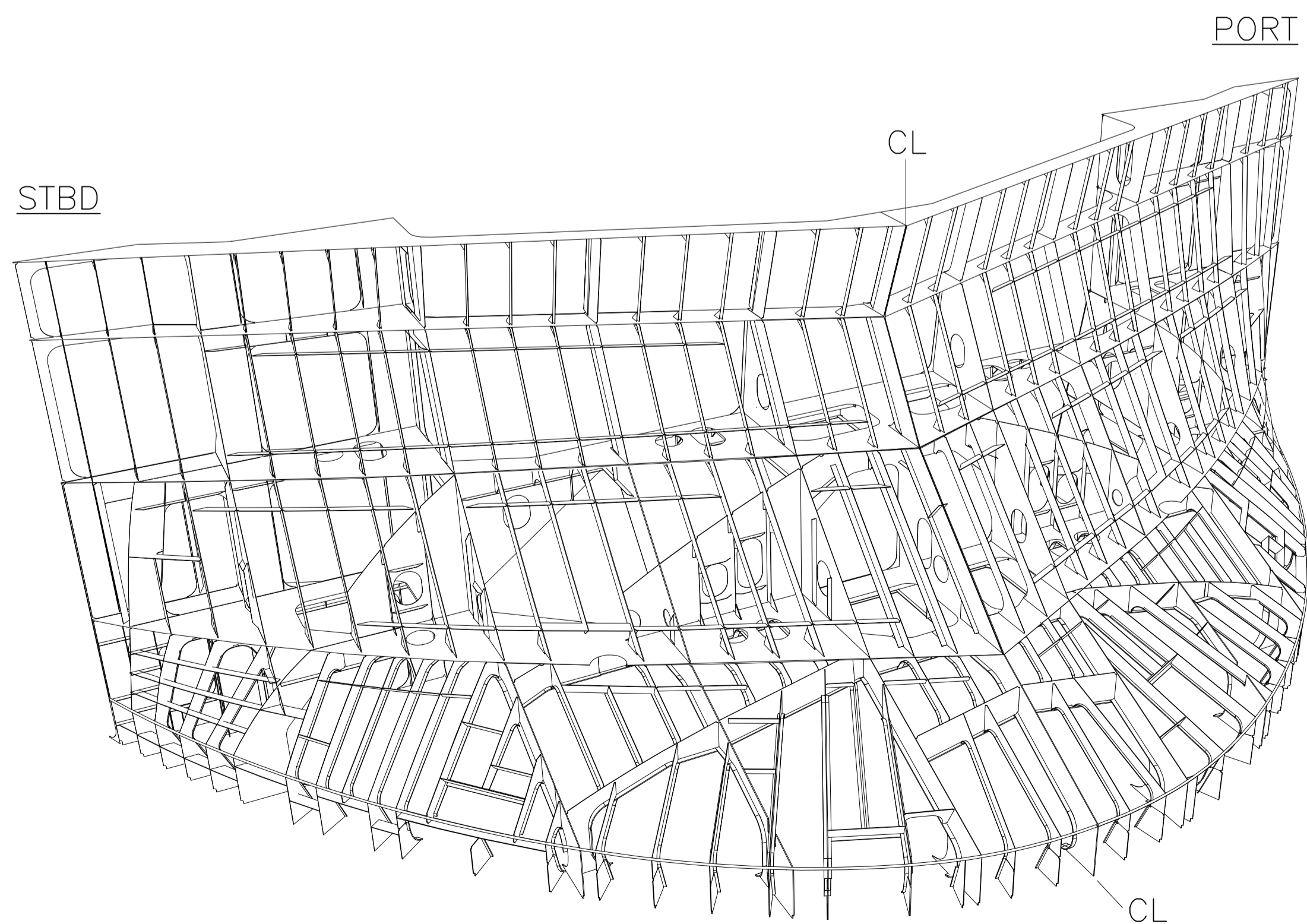
- BOW COVER ISO VIEW - LOOKING AFT / PORT SHELL PLATE NOT SHOWN
